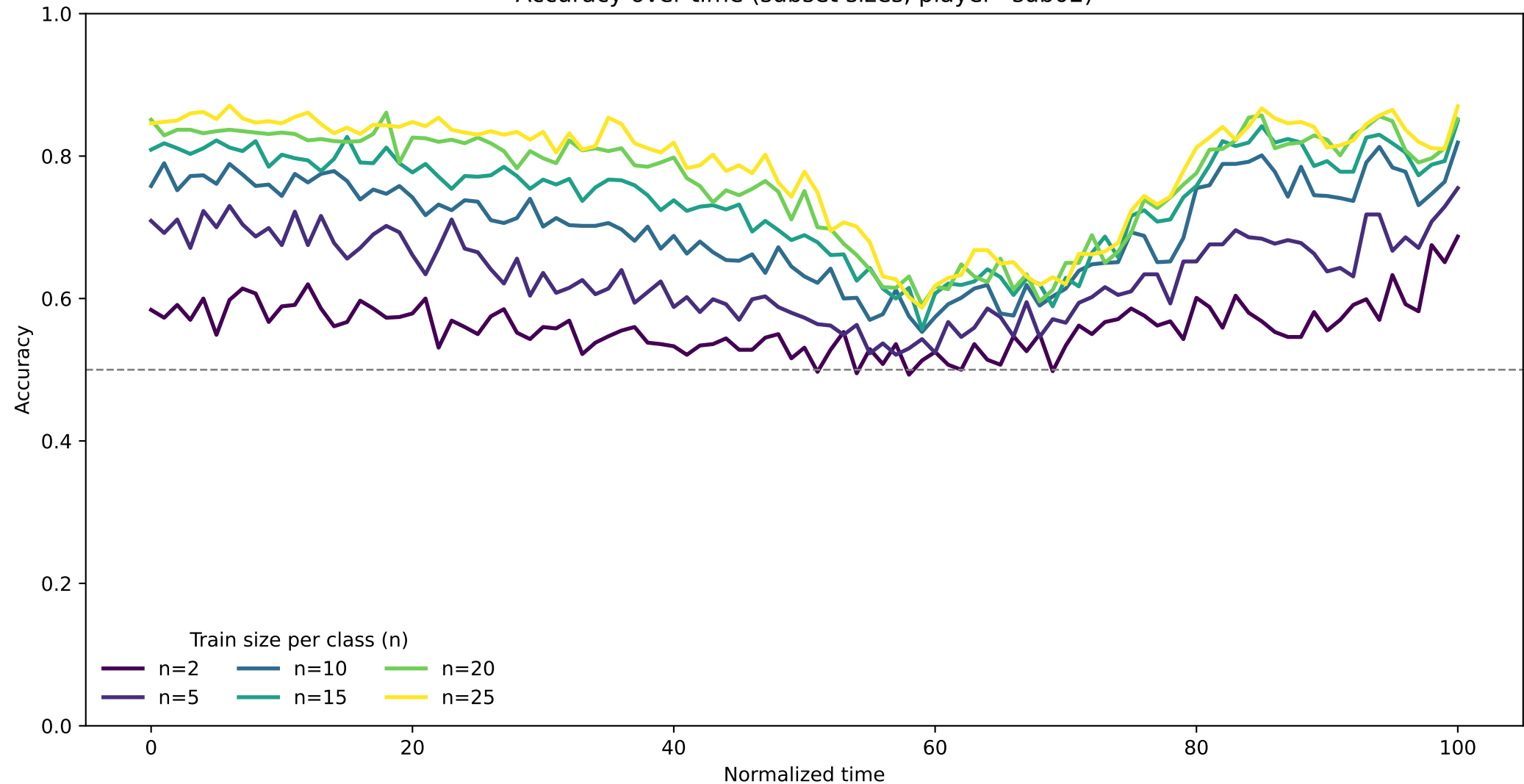
Accuracy over time (subset sizes, player=sub02)
