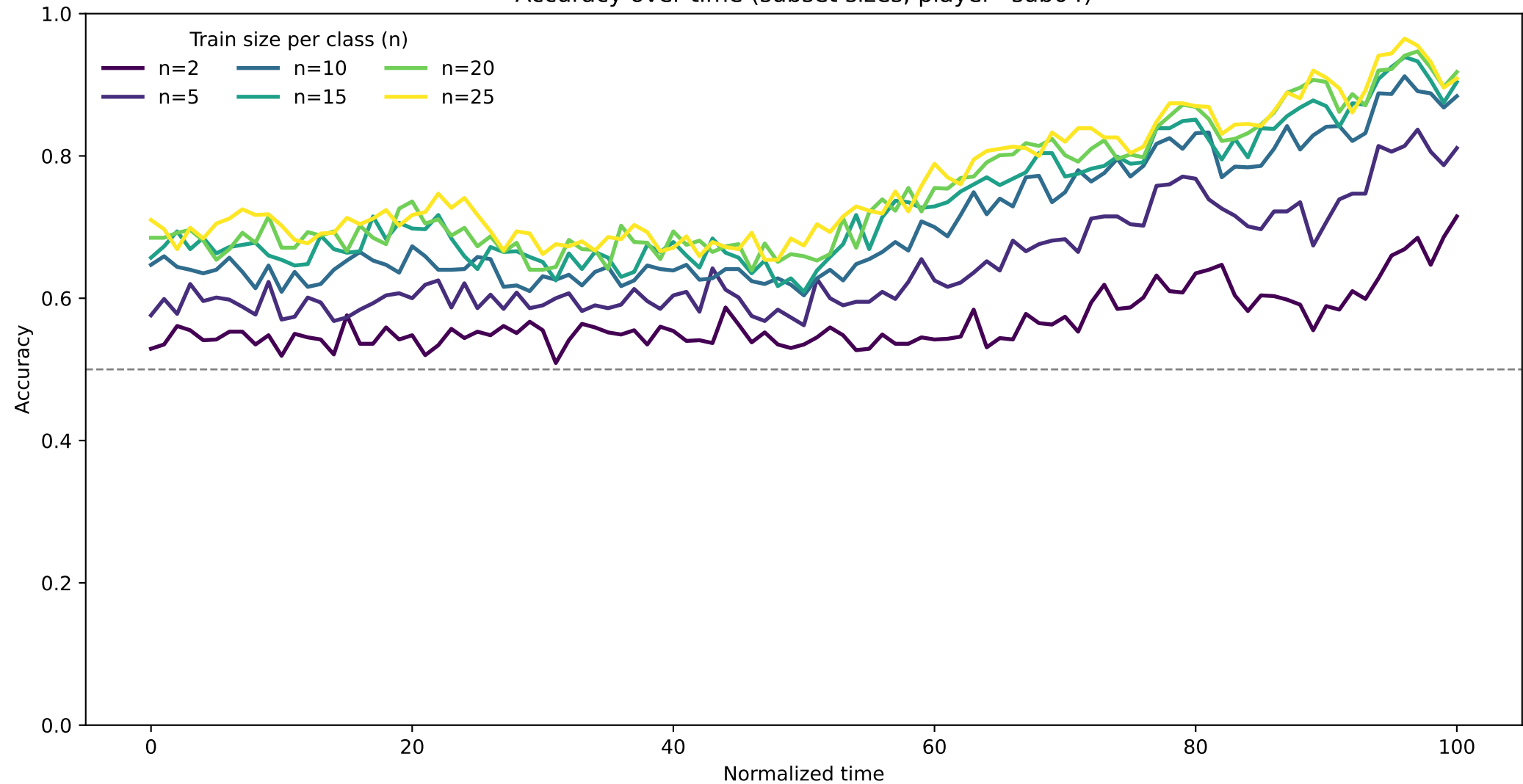
Accuracy over time (subset sizes, player=sub04)
