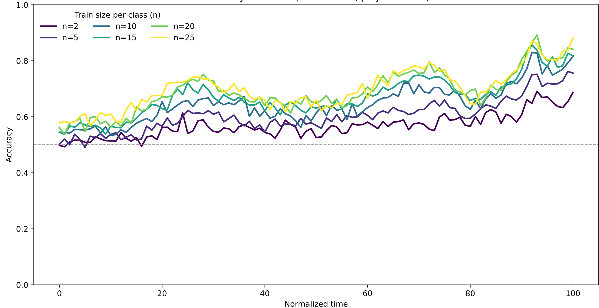
Accuracy over time (subset sizes, player=sub05)
