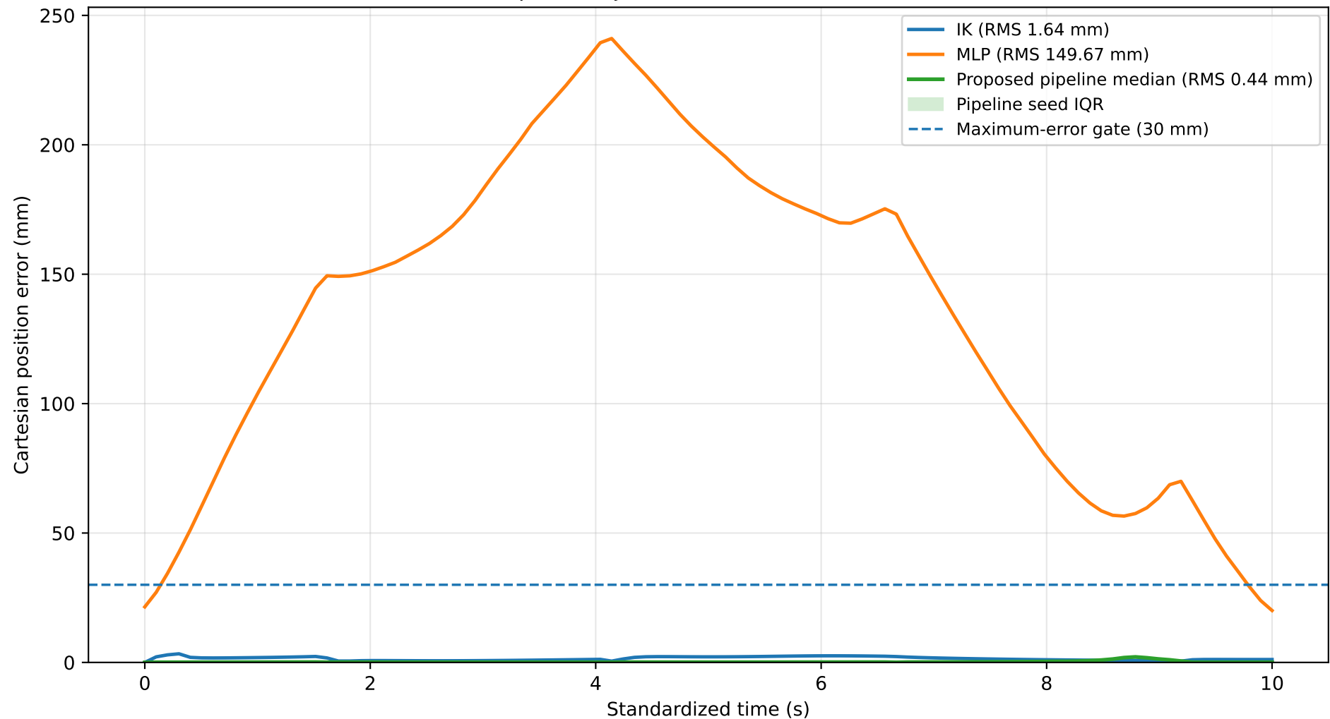
path_0001: Cartesian Tracking Error Over Time Complete trajectories standardized to 10 s
