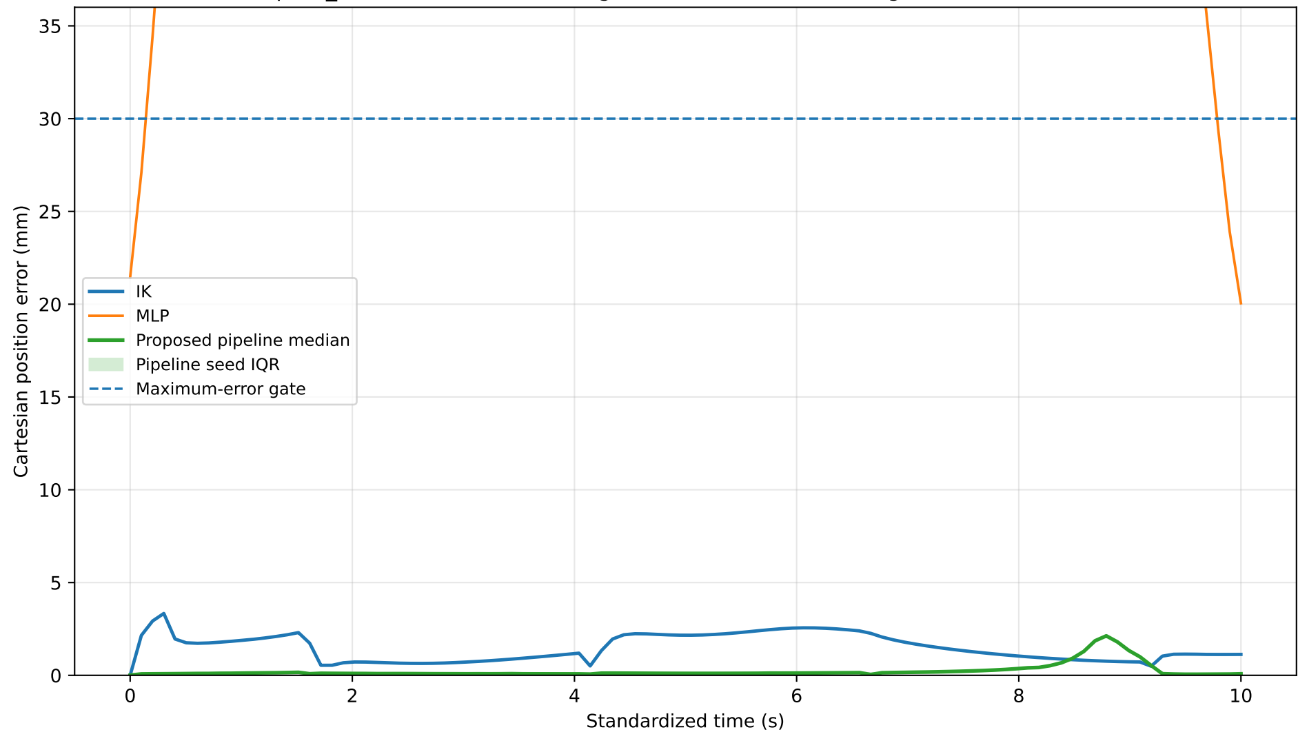
path_0001: Cartesian Tracking Error Over Time (Tracking-Threshold Zoom)
