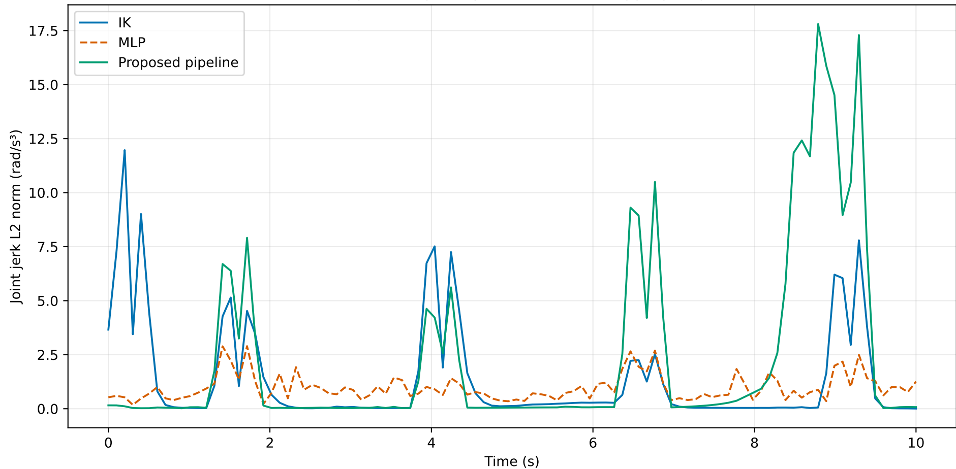
Path 0001: IK vs MLP vs Proposed Pipeline Standardized complete-trajectory duration: 10 s: aggregate jerk over time
