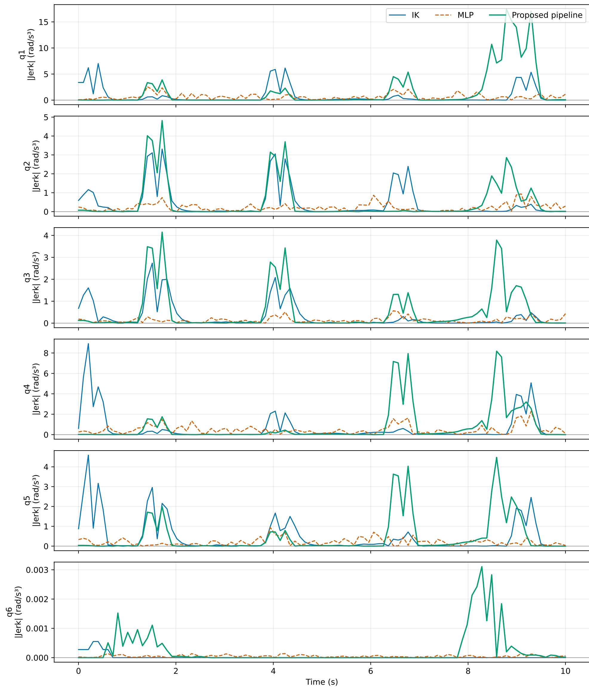
Path 0001: IK vs MLP vs Proposed Pipeline Standardized complete-trajectory duration: 10 s: absolute joint jerk over time
