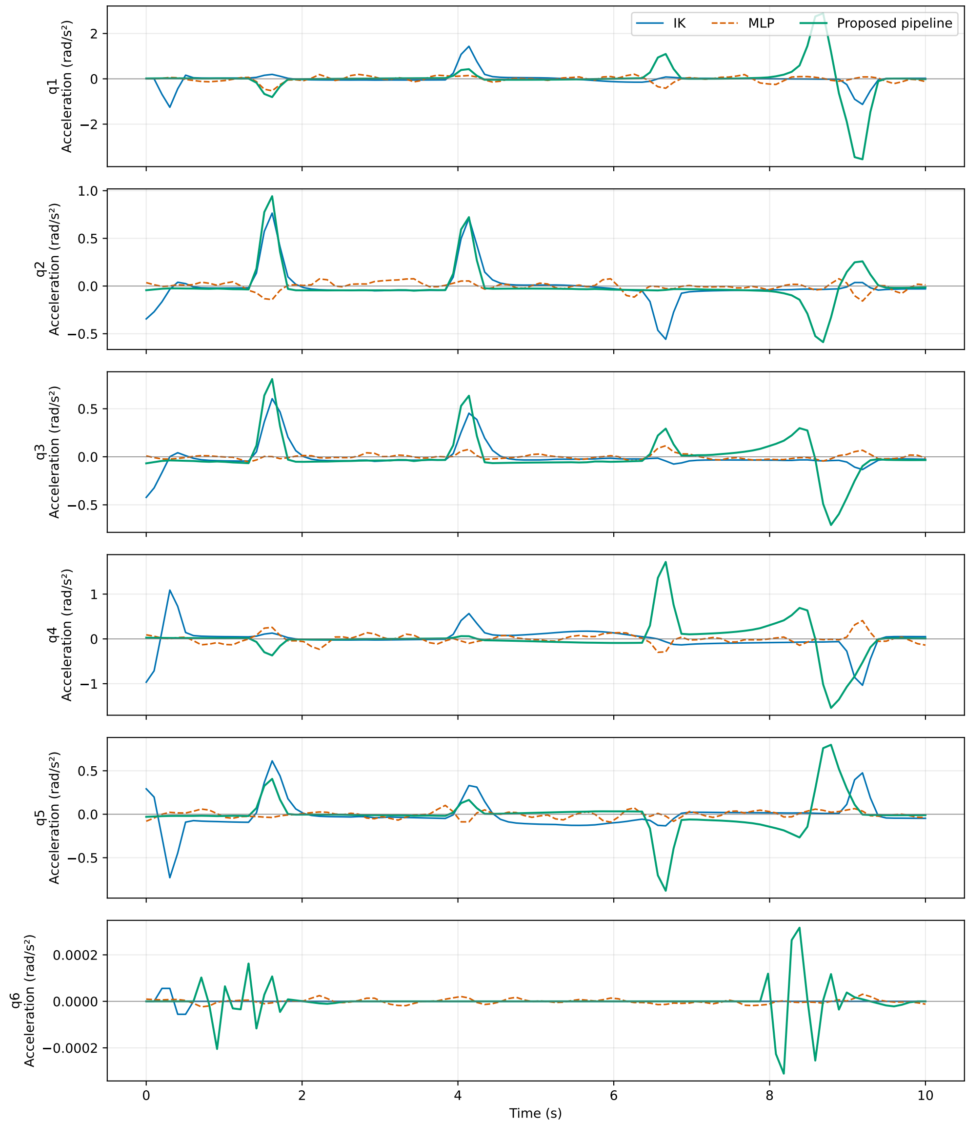
Path 0001: IK vs MLP vs Proposed Pipeline Standardized complete-trajectory duration: 10 s: joint acceleration over time
