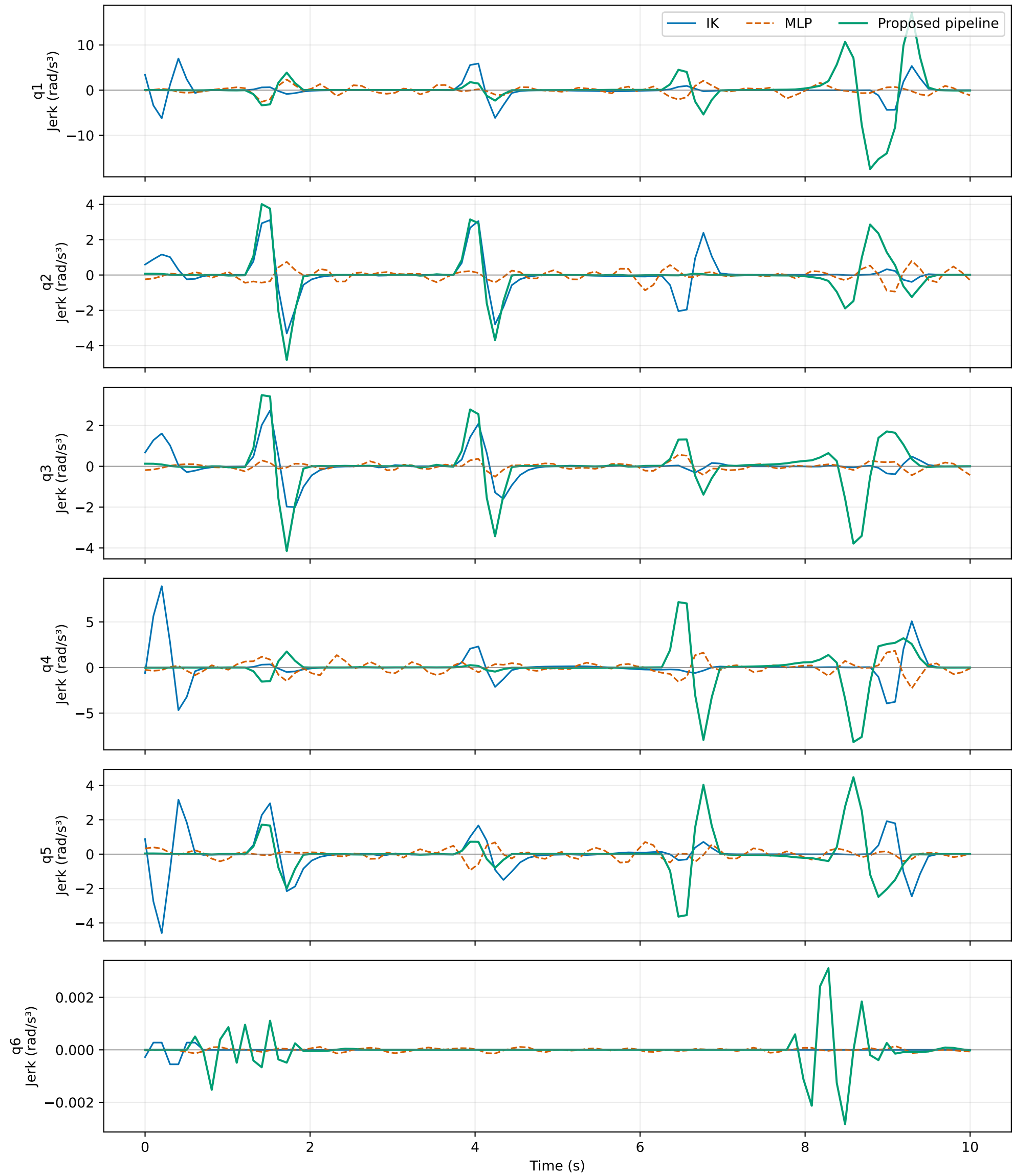
Path 0001: IK vs MLP vs Proposed Pipeline Standardized complete-trajectory duration: 10 s: joint jerk over time
