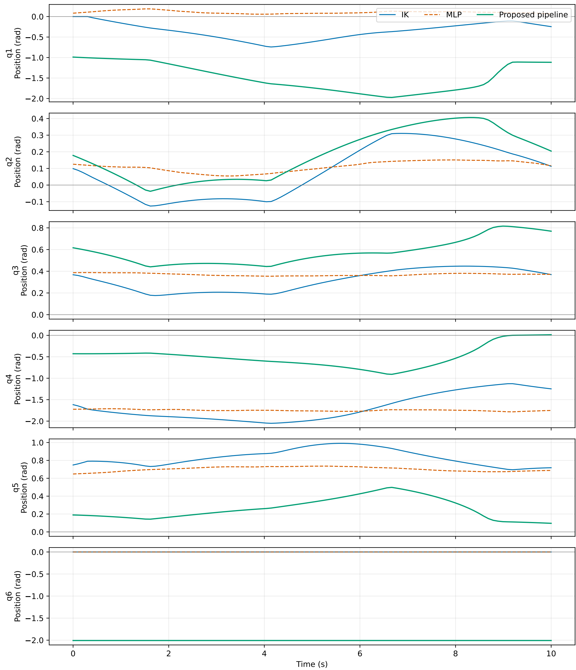
Path 0001: IK vs MLP vs Proposed Pipeline Standardized complete-trajectory duration: 10 s: joint positions over time
