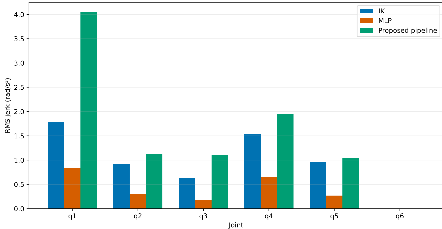
Path 0001: IK vs MLP vs Proposed Pipeline Standardized complete-trajectory duration: 10 s: per-joint RMS jerk
