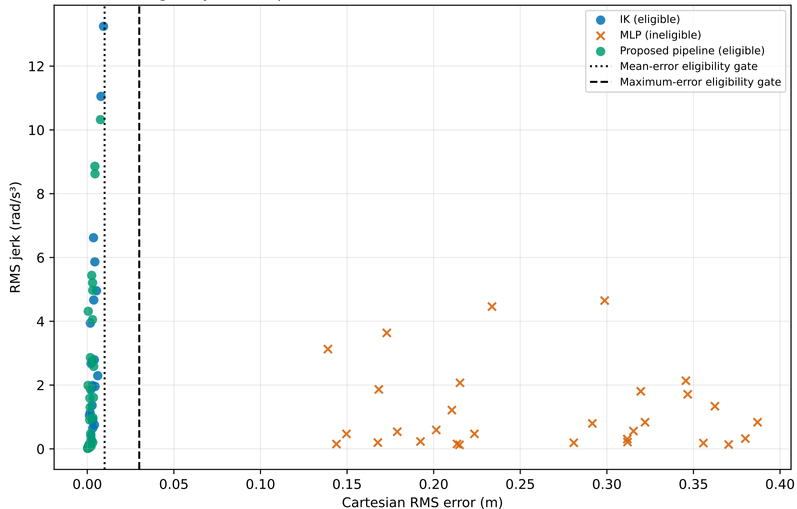
Accuracy-smoothness Pareto view Eligibility uses separate mean and maximum errors; x-axis shows RMS
