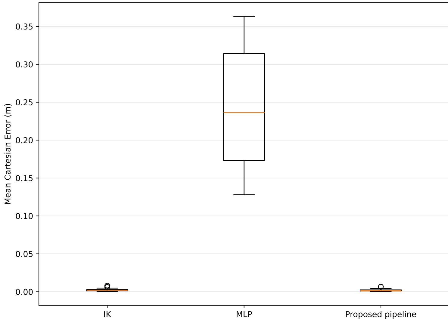
Mean Cartesian Error (m) by Method
