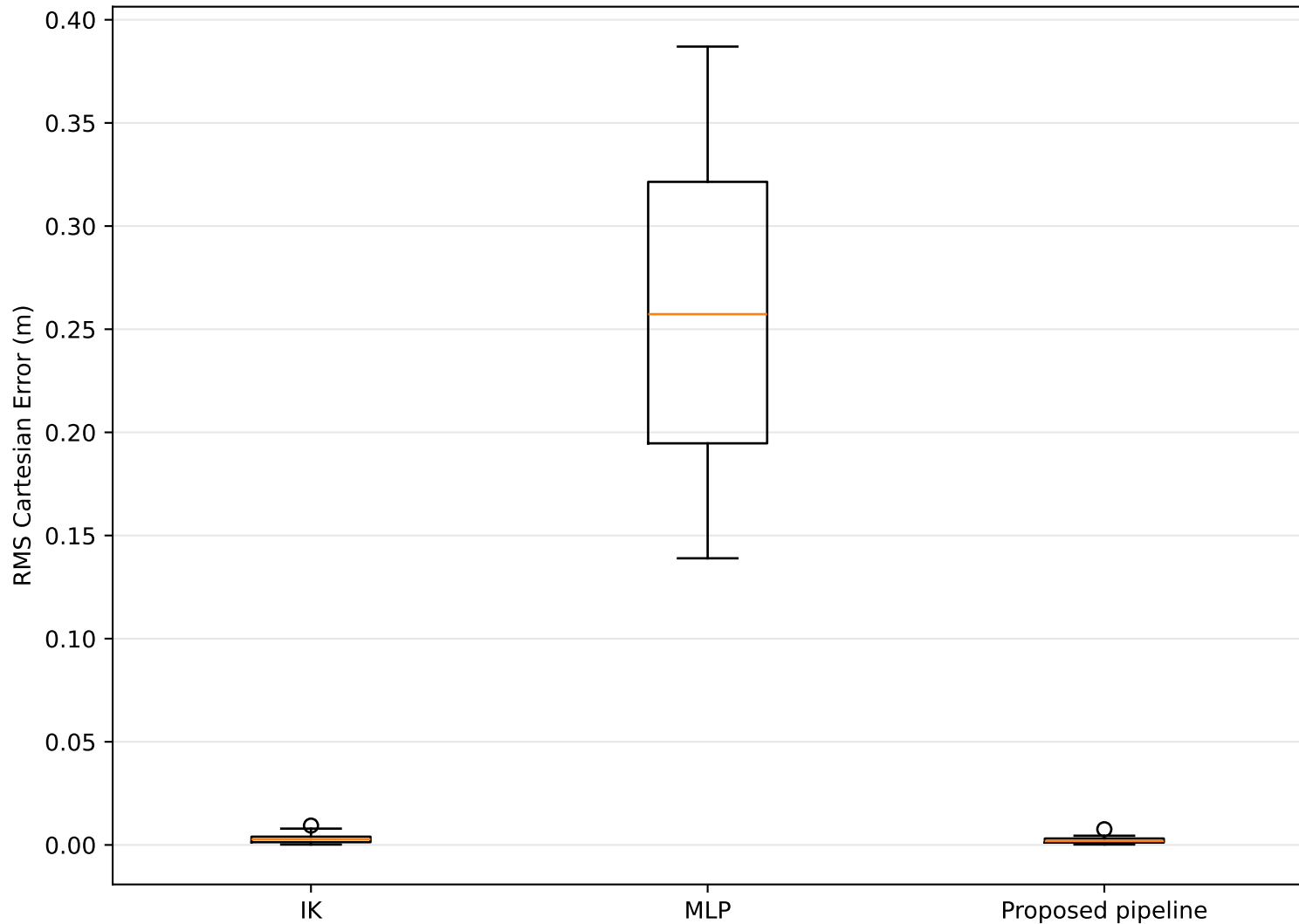
RMS Cartesian Error (m) by Method
