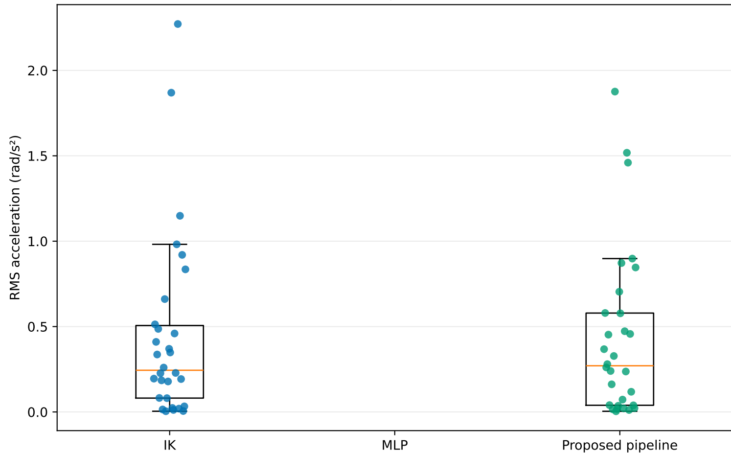
Path-level RMS acceleration ( \text{rad/s}^2 ) Standardized complete duration: 10 s
