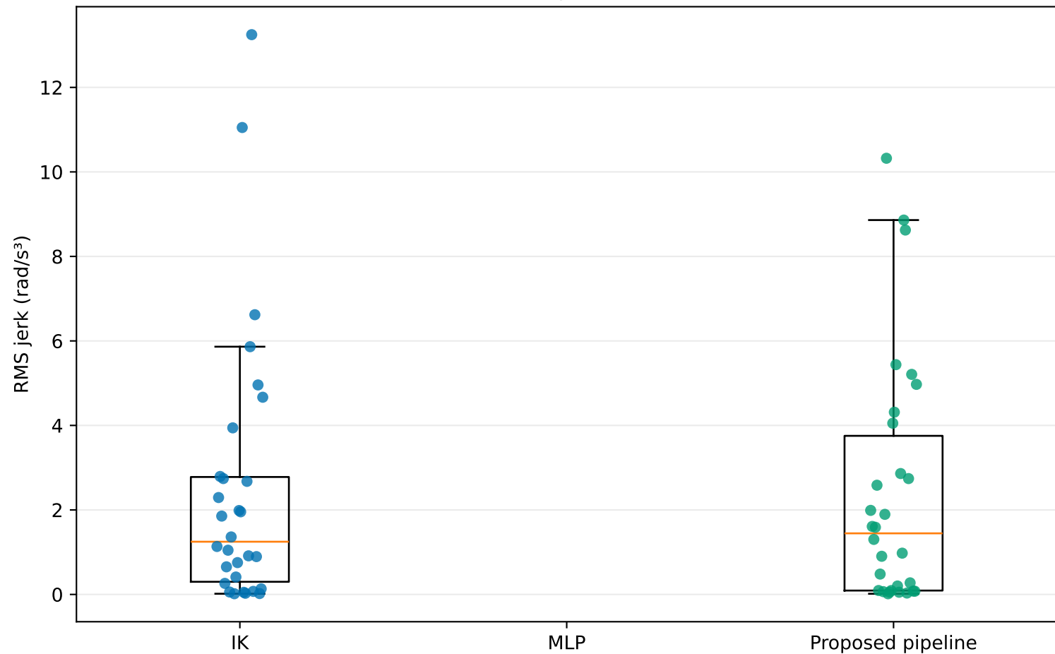
Path-level RMS jerk ( \text{rad/s}^3 ) Standardized complete duration: 10 s
