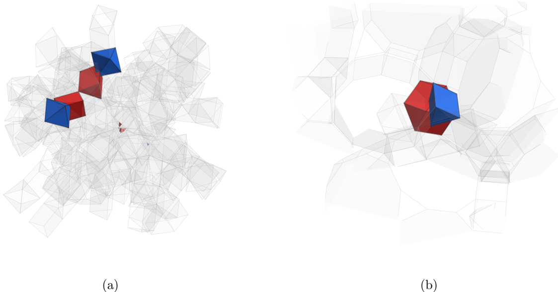
Figure 2: The two ways the unfolding fails. (a) The runcinated 24-cell at its best root: 3 of its 240 cells intersect a partner, the fewest over all 240 roots, and no root does better than 3. (b) The runcitruncated 120-cell at one of its 70 failing roots, where a single pair of cells intersects; nearby cells are drawn faintly for context. In both panels the two members of an intersecting pair are drawn in different colors.
