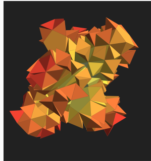
Grand antiprism, one valid net
