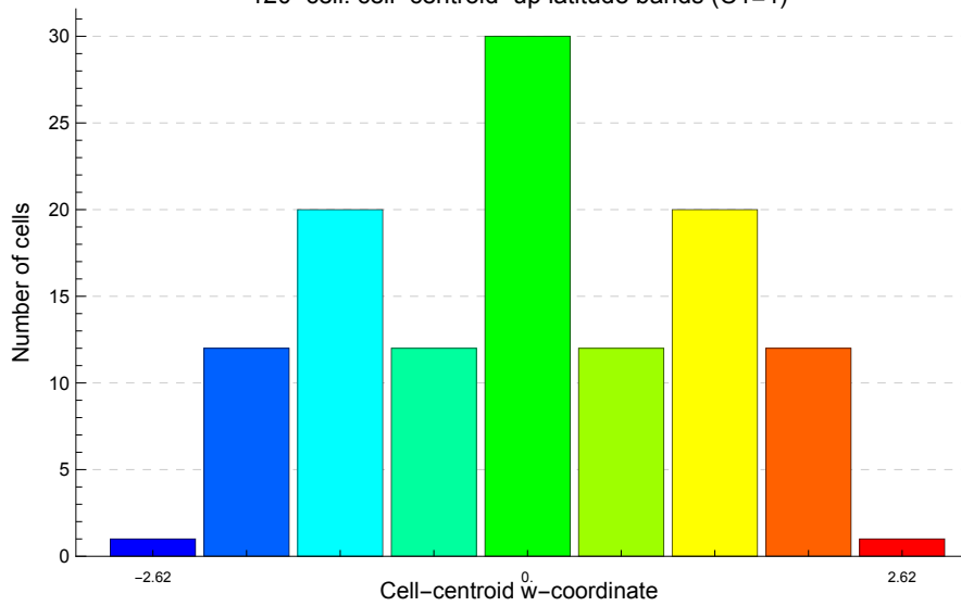
120-cell: cell-centroid-up latitude bands (C1=1)
