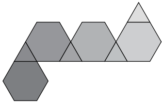
Truncated Tetrahedron (3.6.6)
