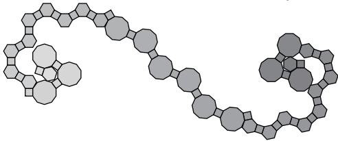
Truncated Icosidodecahedron (4.6.10)
