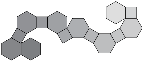
Truncated Octahedron (4.6.6)
