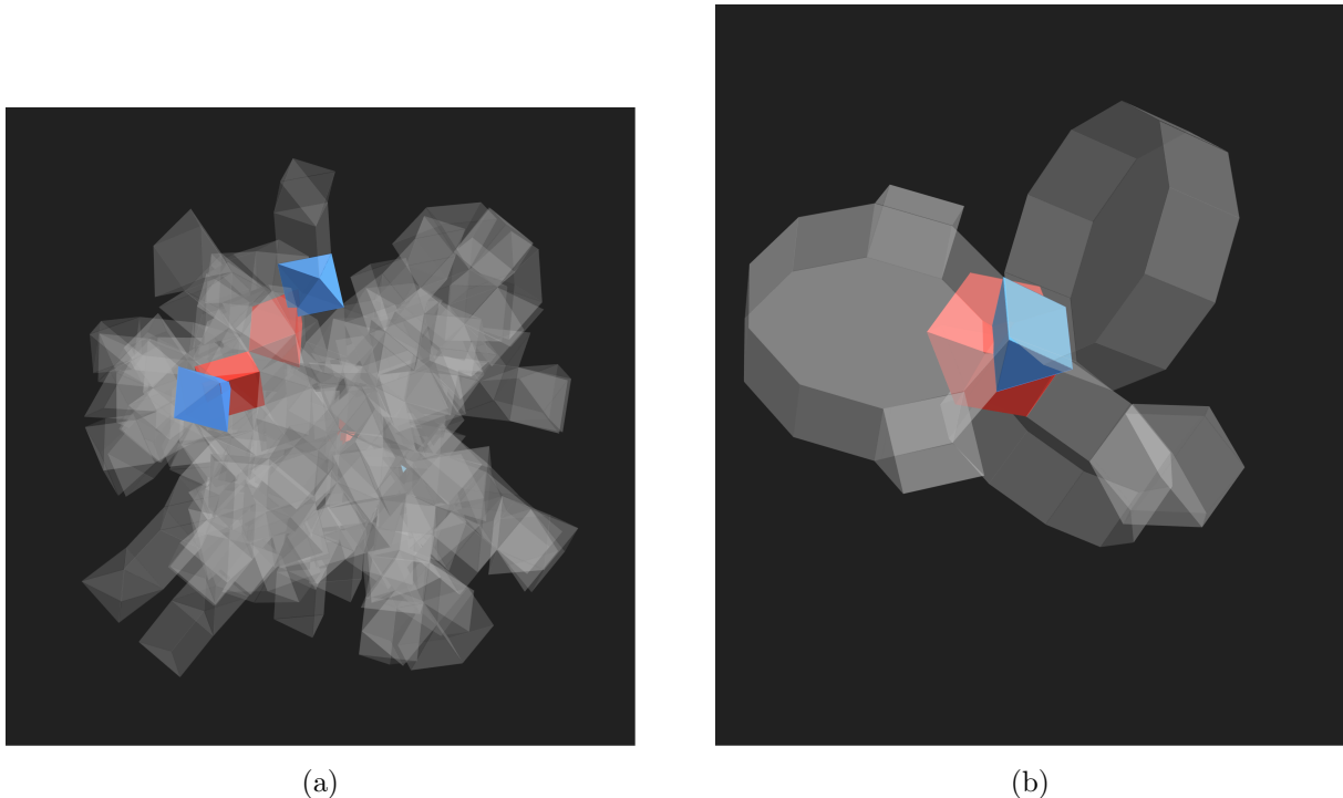
Figure 2: The two ways the unfolding fails. (a) The runcinated 24-cell at its best root: 3 of its 240 cells intersect a partner, the fewest over all 240 roots, and no root does better than 3. (b) The runcitruncated 120-cell at one of its 70 failing roots, where a single pair of cells intersects; nearby cells are drawn faintly for context. In both panels the two members of an intersecting pair are drawn in different colors.
