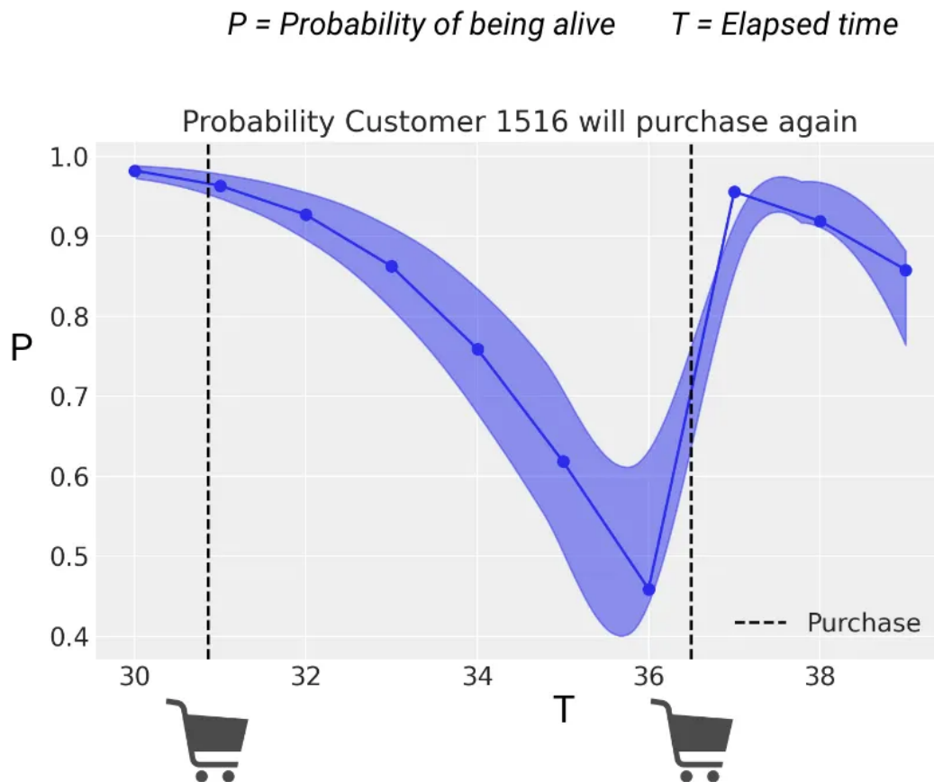
Figure 9: P(\text{alive}) decays with time since last purchase, then resets on a new purchase.
