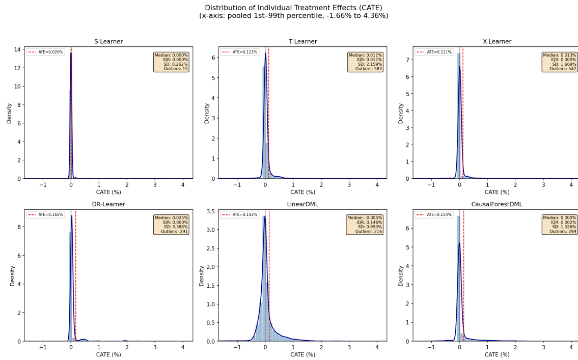
Figure 4: CATE distributions across six meta-learners on a shared x-axis (1st–99th pct).
