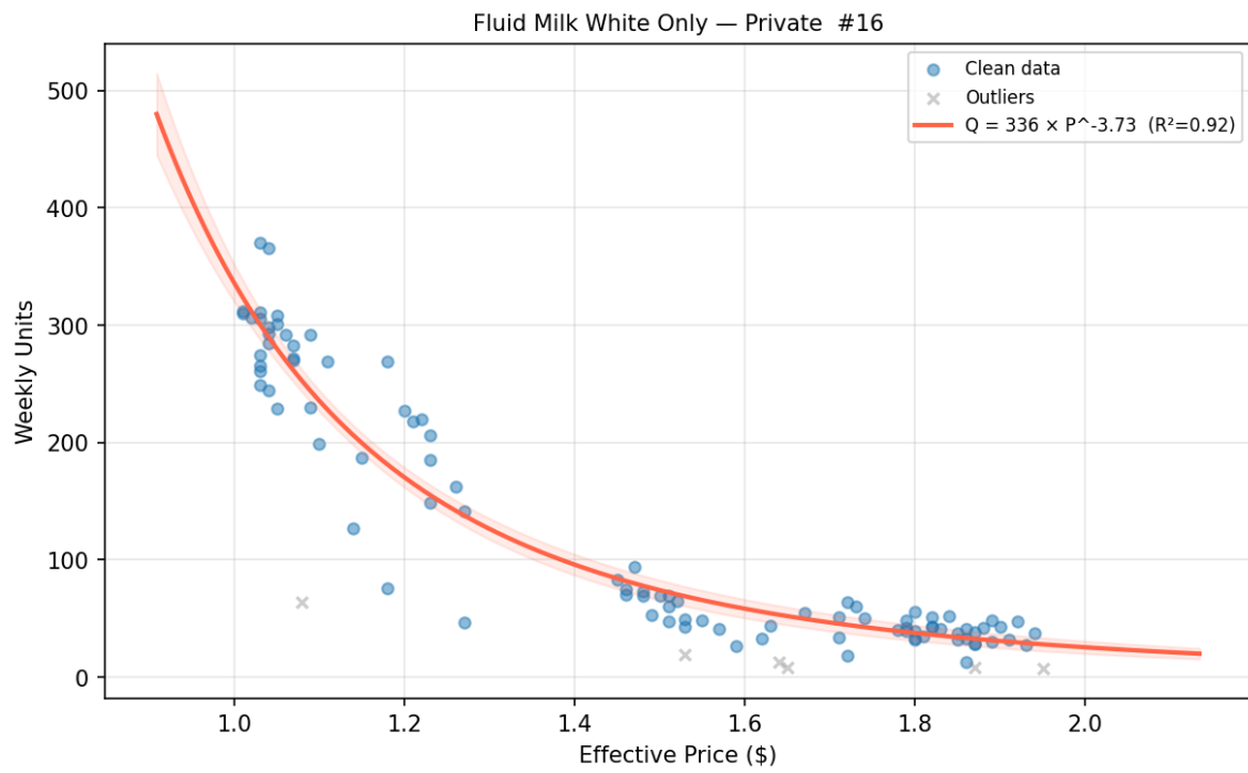
Figure 1: Price–quantity scatter and fitted power curve for a top-selling Fluid Milk SKU (Dunnhumby).
