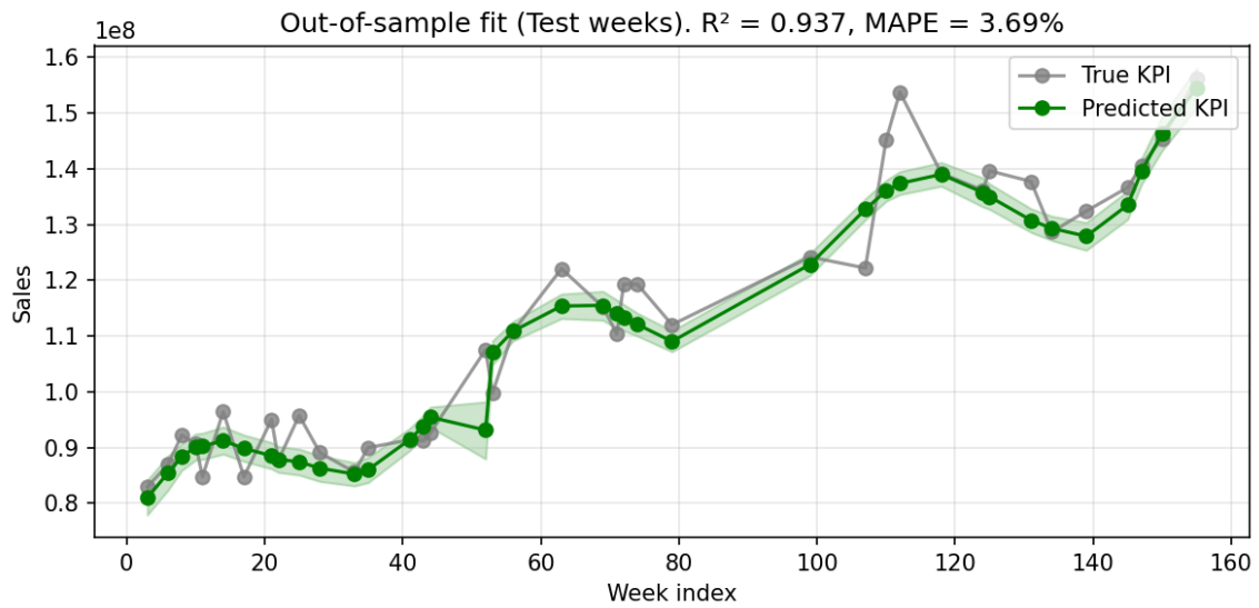
Figure 9: Out-of-sample model fit: predicted vs. actual sales on the random-holdout weeks ( R^2 = 0.94 ).
