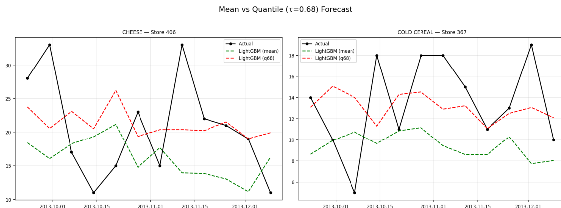
Figure 4: Quantile forecasts under asymmetric costs: optimal bias upward when stockout > overstock.
