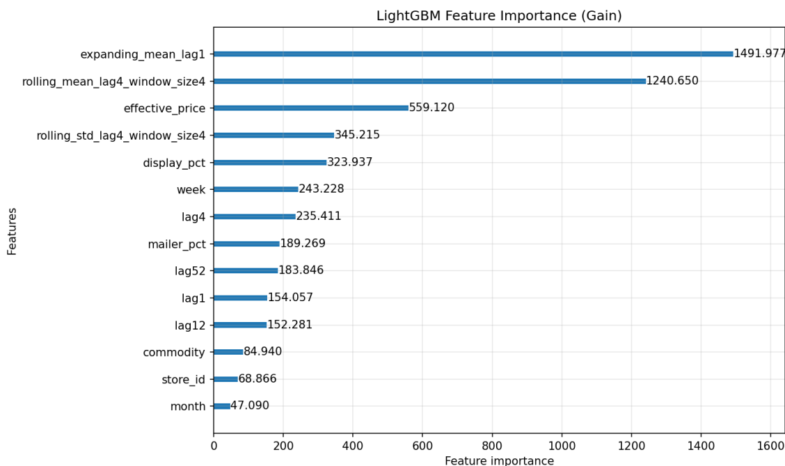
Figure 1: LightGBM feature importance (gain) for Dunnhumby grocery data.
