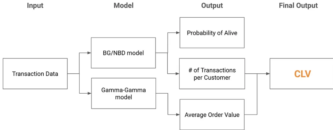
Figure 7: BTYD framework: BG/NBD ( P(\text{alive}) , transactions) + Gamma-Gamma (AOV) \rightarrow CLV.
