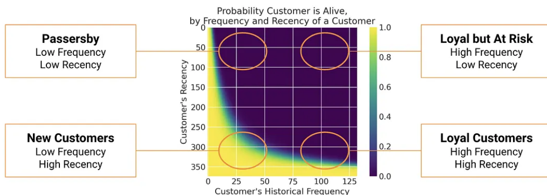
Figure 11: Probability Alive matrix by purchase frequency (x) and recency (y).
