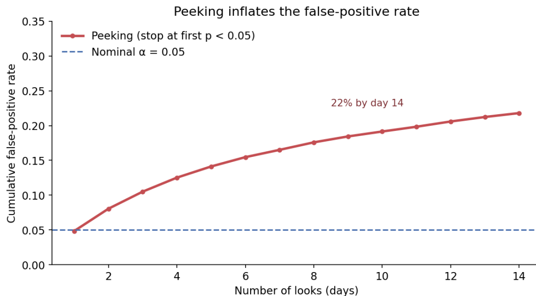
Figure 3: Peeking inflates the false-positive rate.
