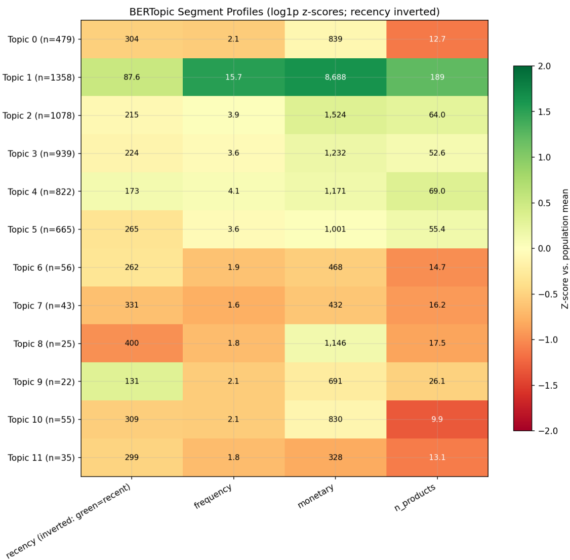
Figure 4: A segment profile heatmap.
