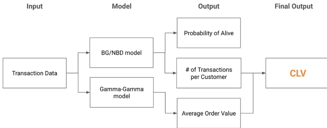
Figure 7: The BTYD framework: BG/NBD plus Gamma-Gamma.
