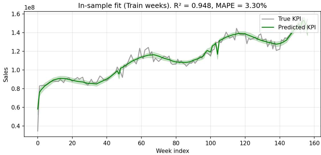
Figure 8: In-sample model fit: predicted vs. actual sales (random-holdout train period; R^2 = 0.95 ).
