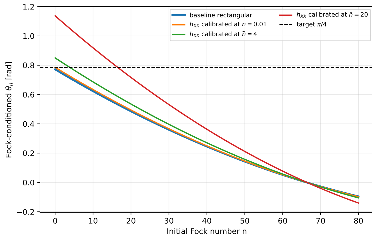
Fock-resolved XX angle and thermal angle-dispersion prediction
