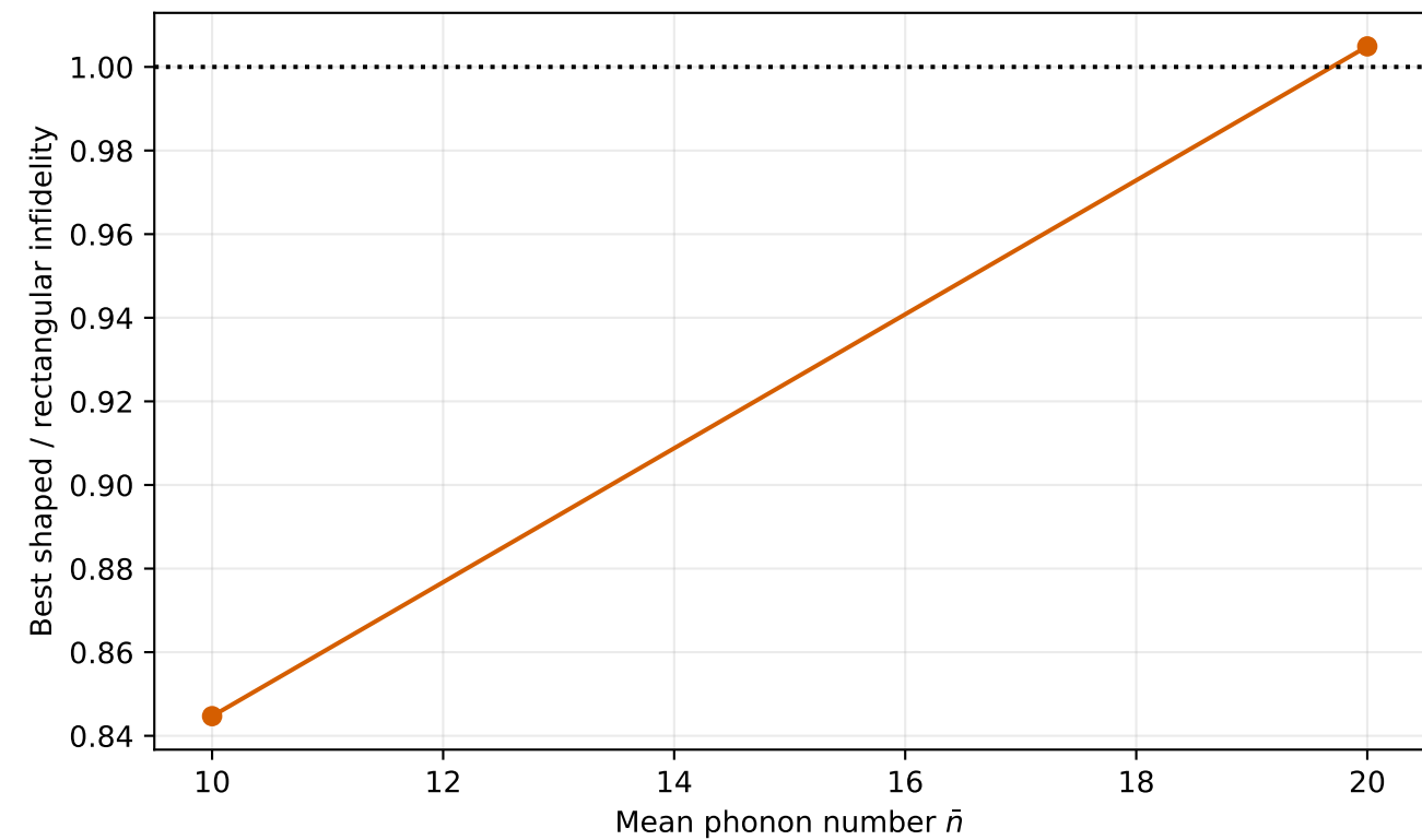
Coherent-to-stochastic crossover
