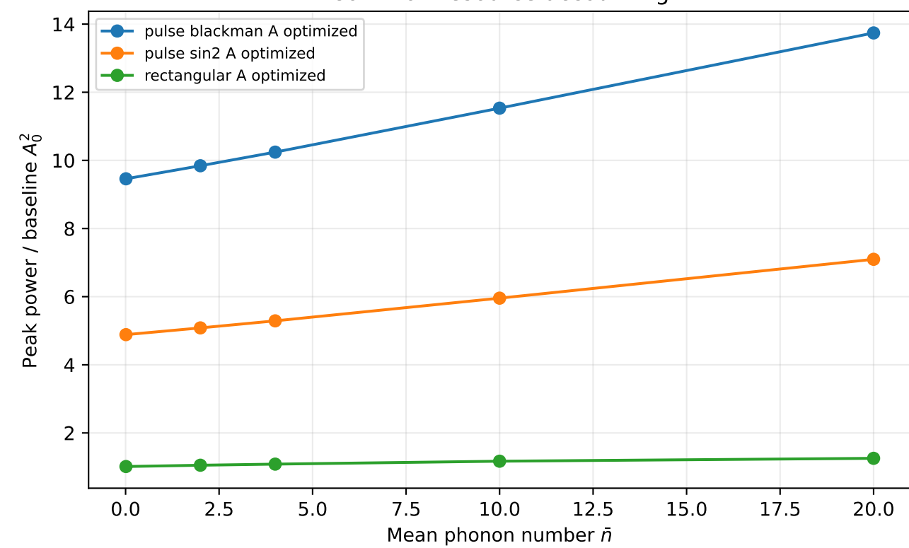
Coherent-to-stochastic crossover
