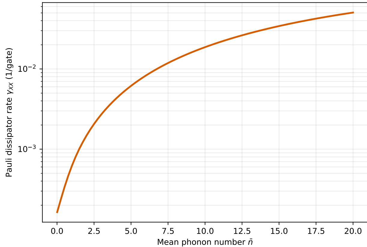
Stochastic Pauli-XX generator component
