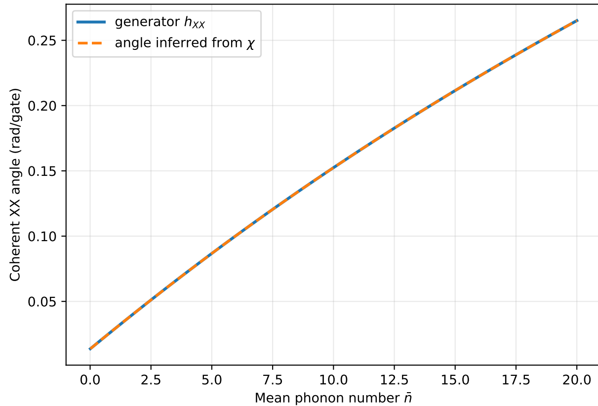
Hamiltonian-type correlated XX error
