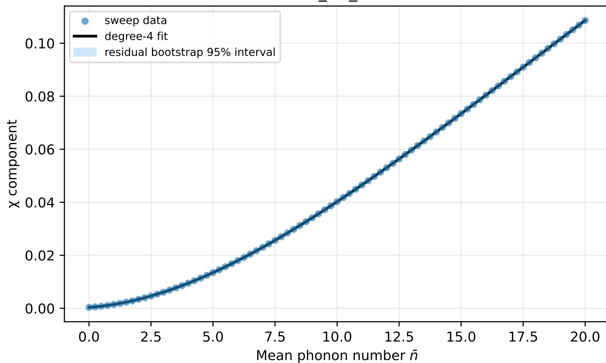
chi_XX_XX
