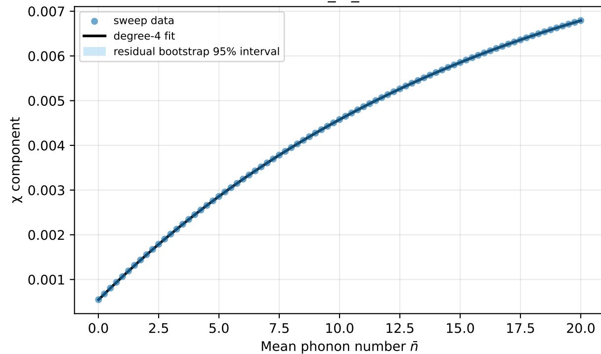
chi_IX_IX
