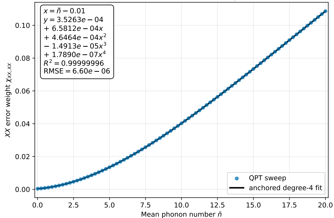
Pauli XX error weight \chi_{XX,XX}
