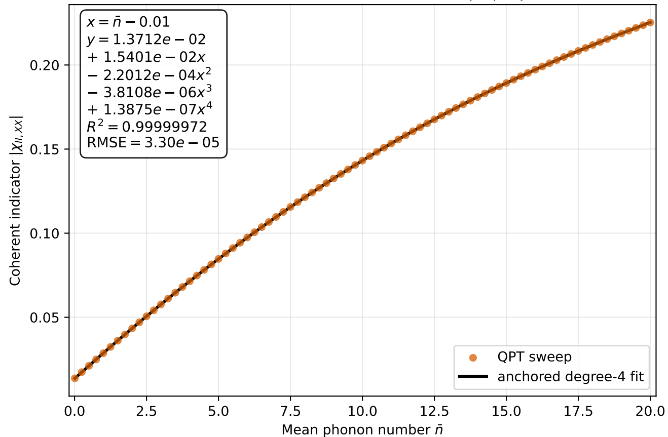
Coherent XX error indicator |\chi_{II,XX}|
