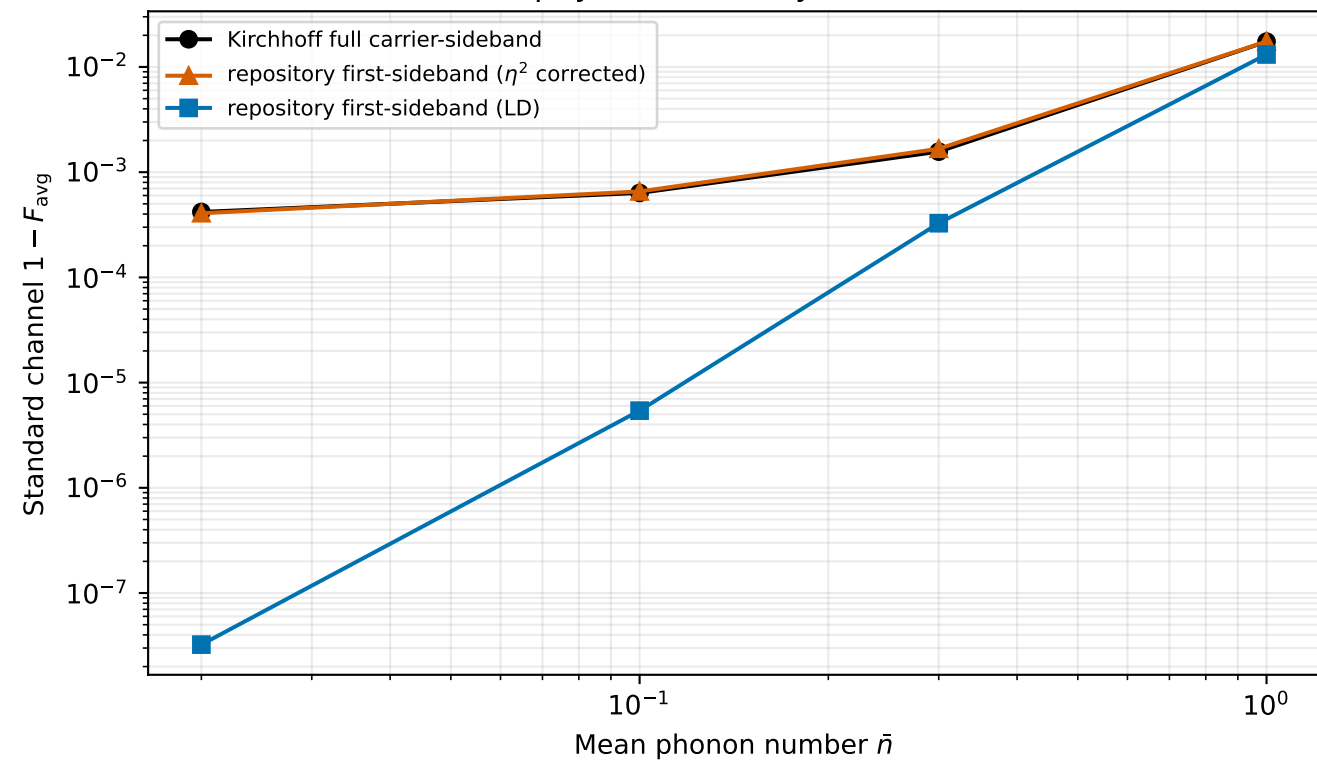
Residual physical infidelity after calibration
