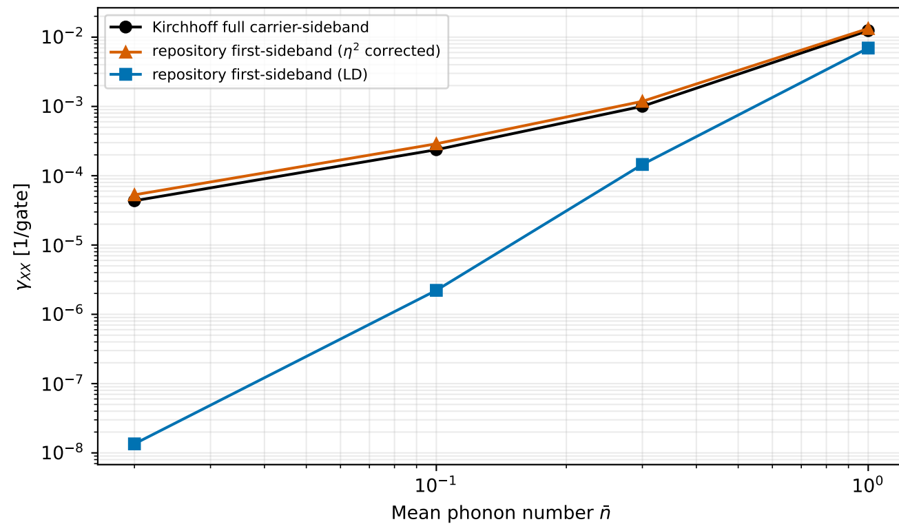
Stochastic XX error after h_{XX} calibration
