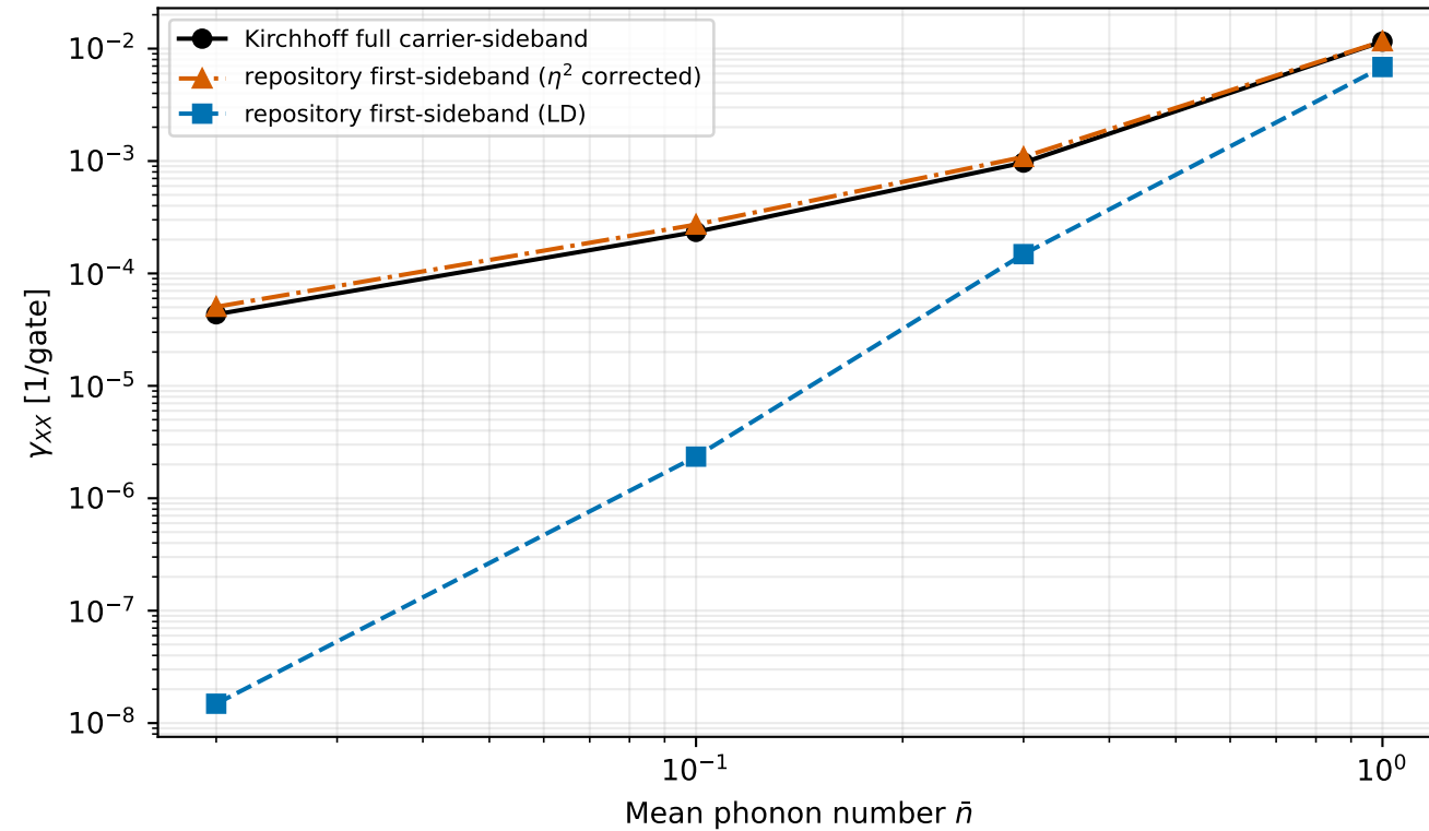
Stochastic XX error at Omega_4
