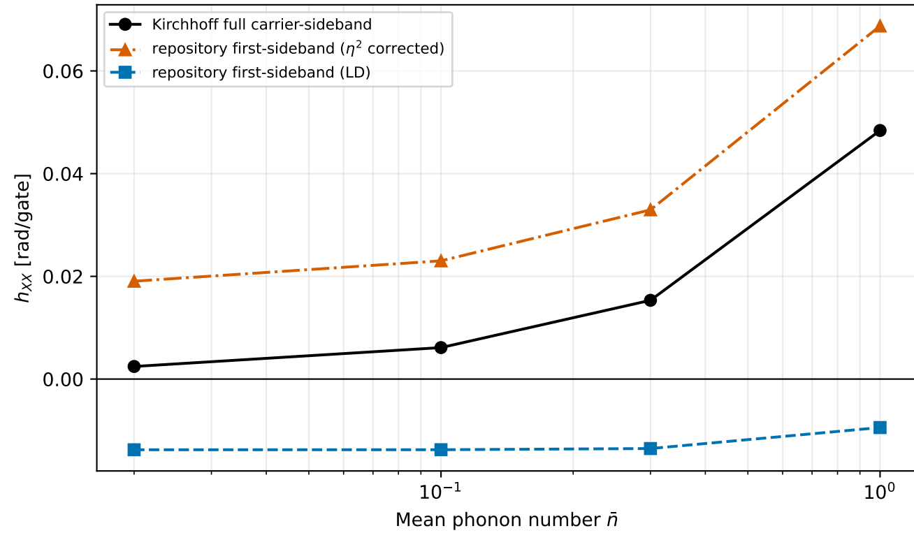
Coherent XX error at Omega_4
