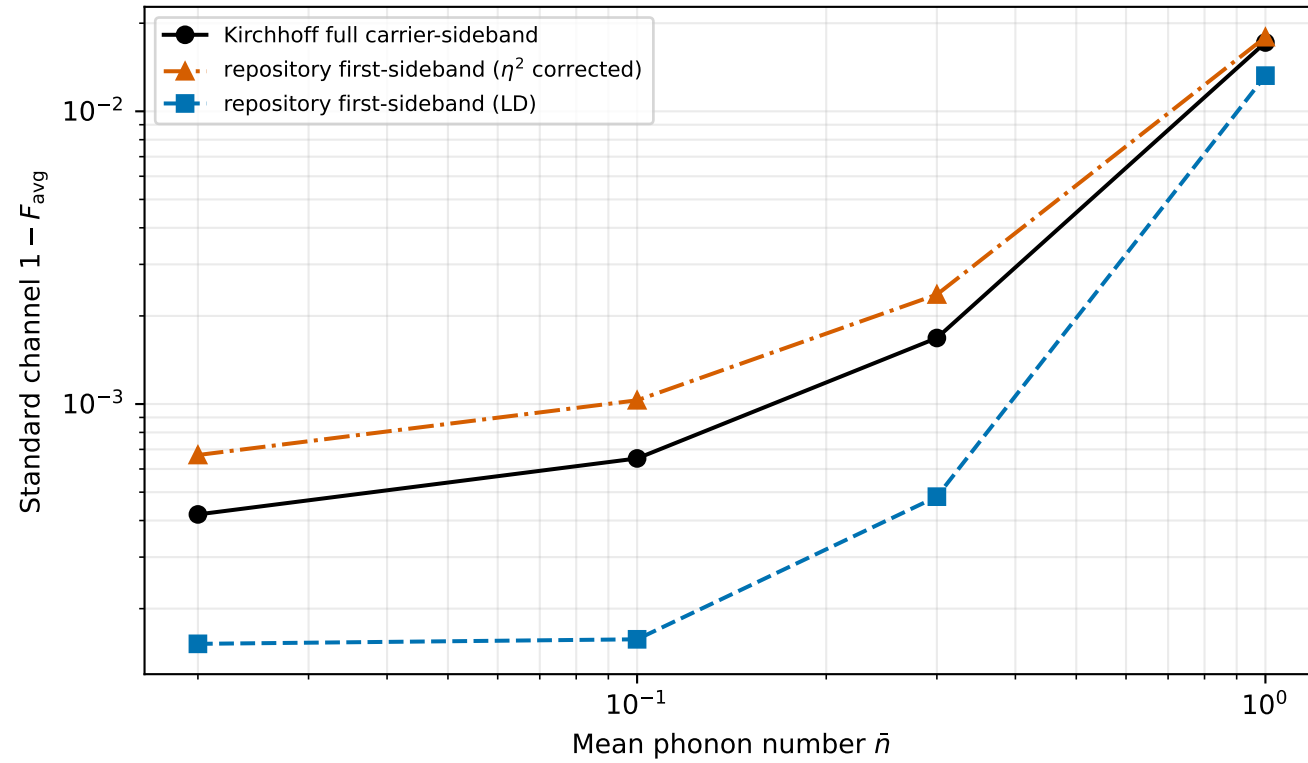
Coherent-limit infidelity at Omega_4
