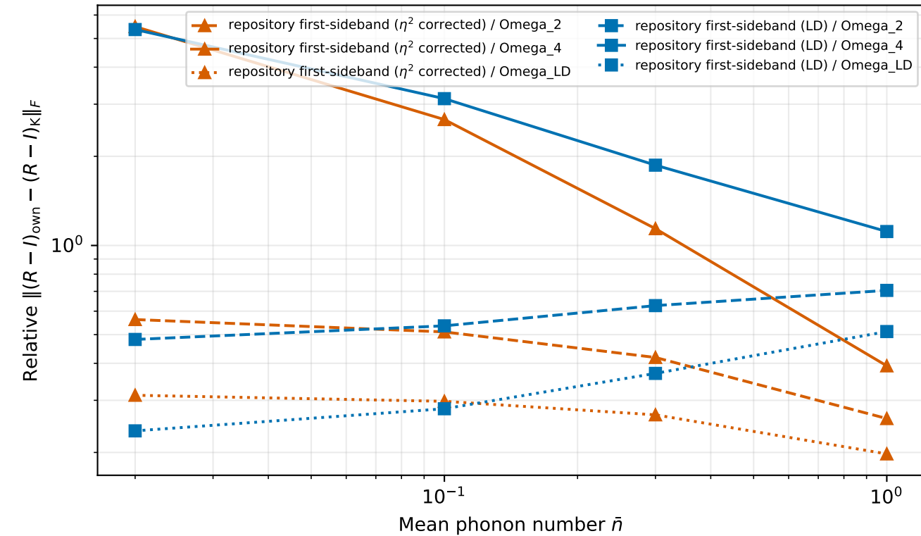
Error-channel PTM mismatch
