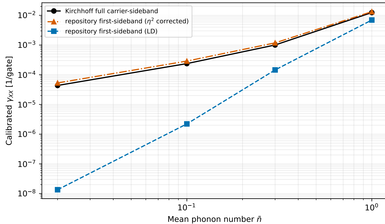
Structural stochastic XX error after angle calibration
