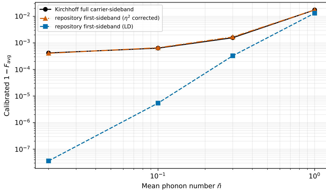
Residual channel infidelity after angle calibration
