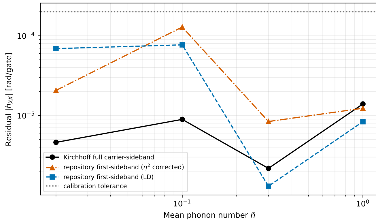
Residual coherent XX error
