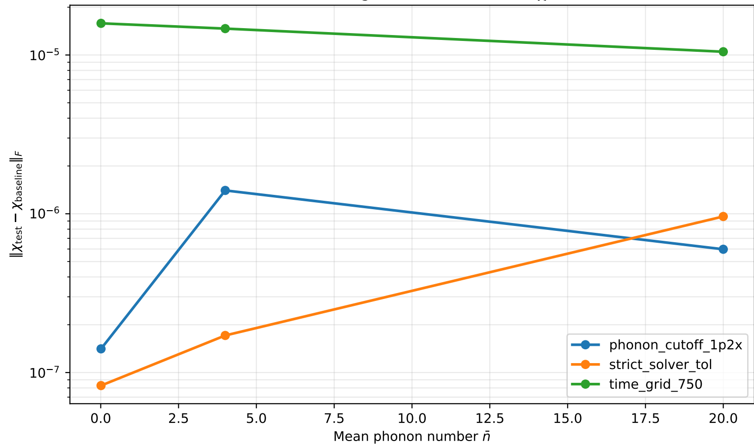
Numerical convergence of the full error \chi matrix
