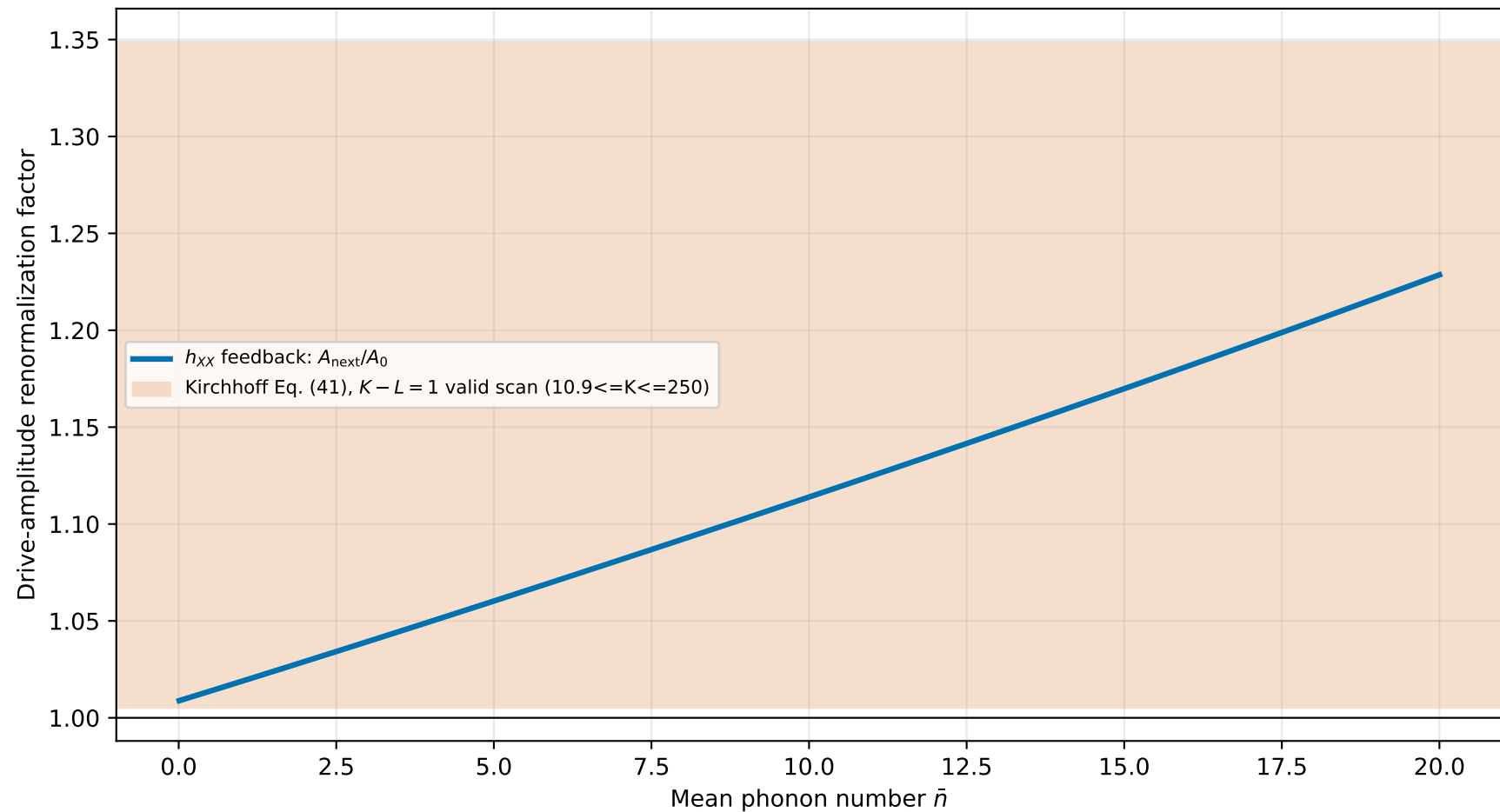
Temperature-adaptive h_{XX} calibration vs Kirchhoff formula
