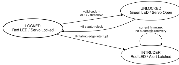
Figure 3: State machine
