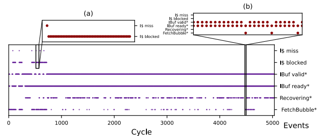
Fig. 3: Cycle-accurate trace of Frontend events for mergesort.
