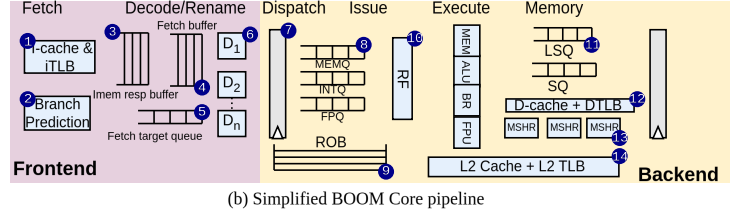
Fig. 2: Core pipelines with marked performance event sources.
