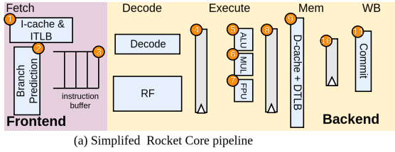
Fig. 2: Core pipelines with marked performance event sources.
