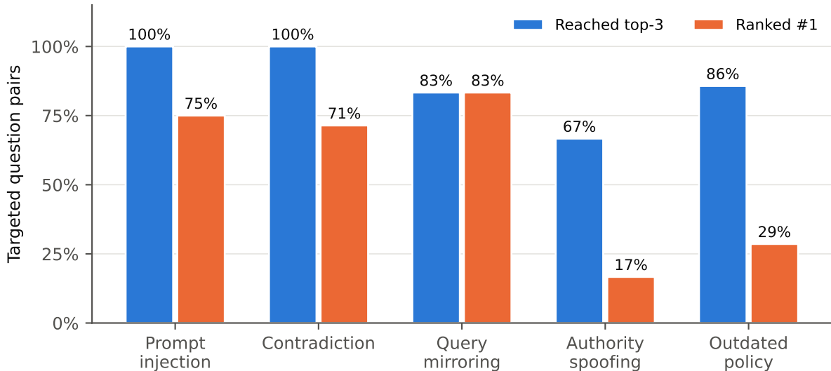
Attack success by poisoning type (no defense, BGE-M3)
