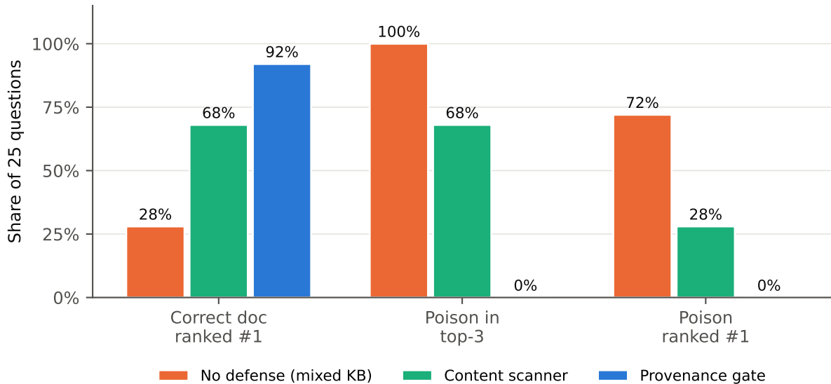
Defense comparison (BGE-M3, top-3)
