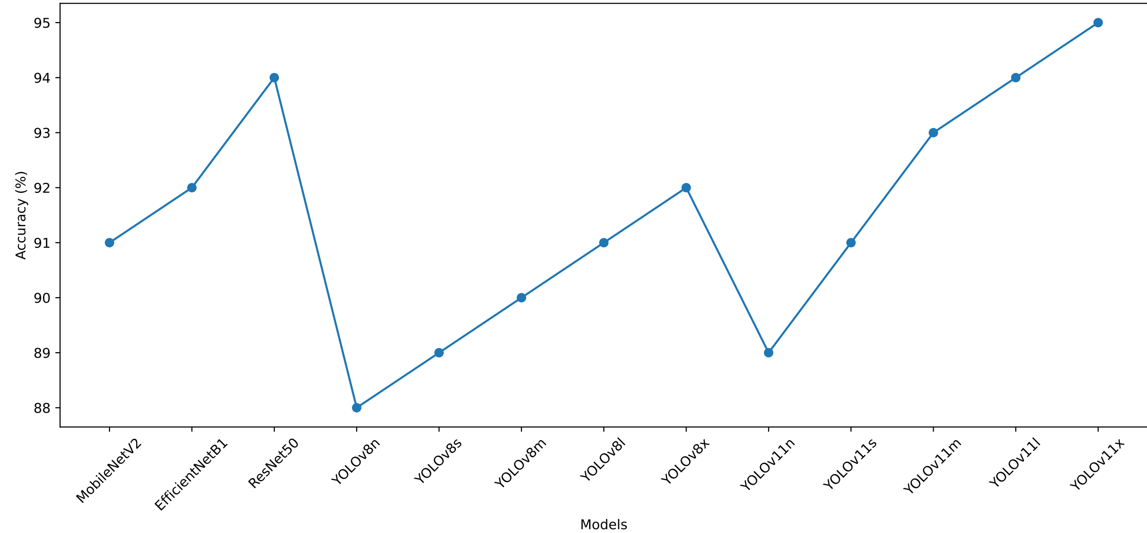
Accuracy Comparison
