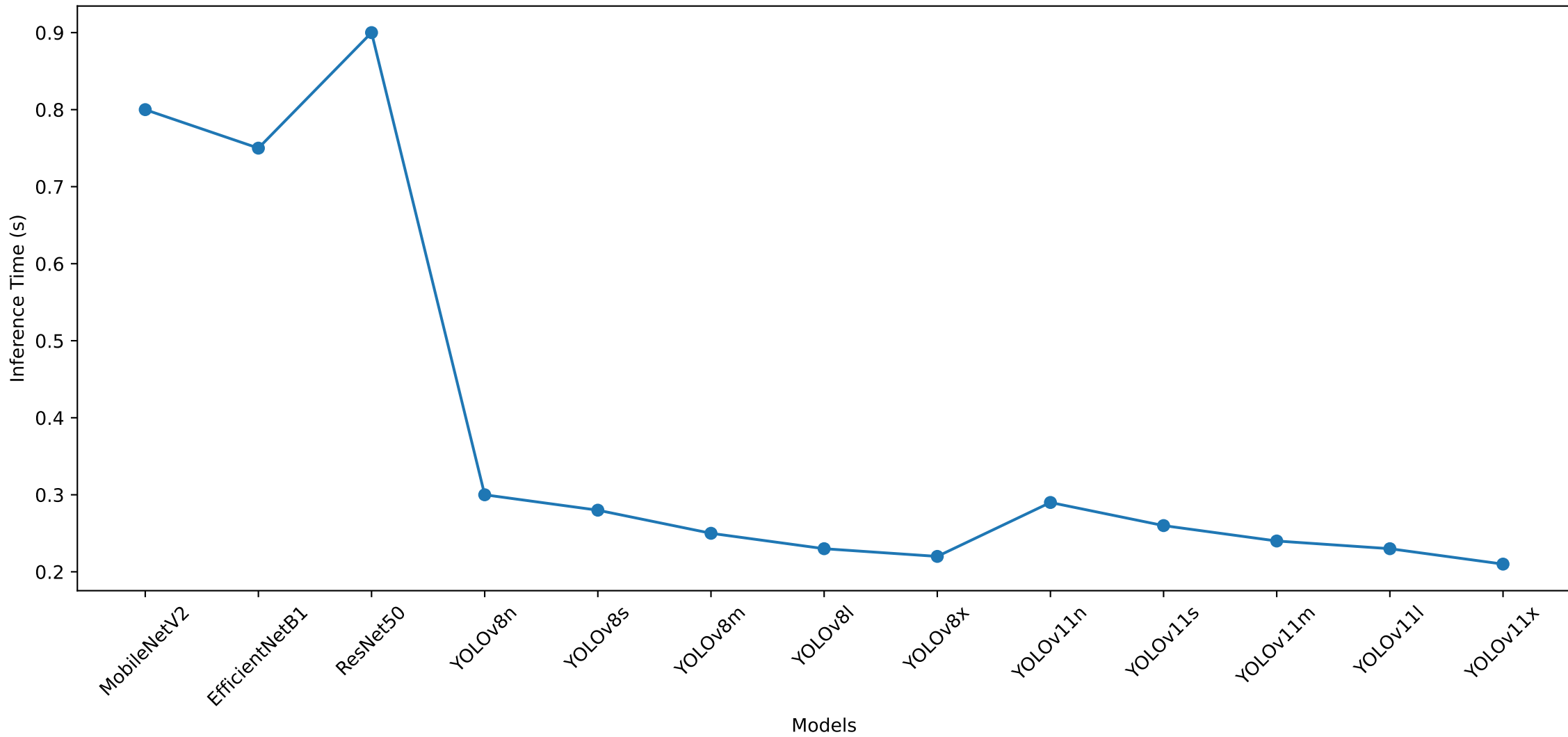
Inference Time Comparison
