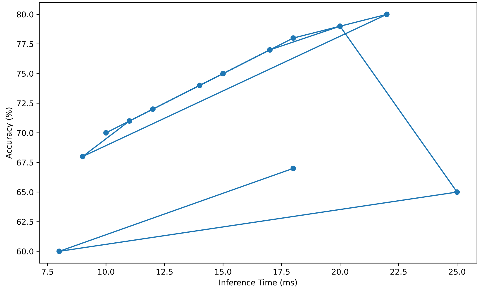
Accuracy vs Inference Time
