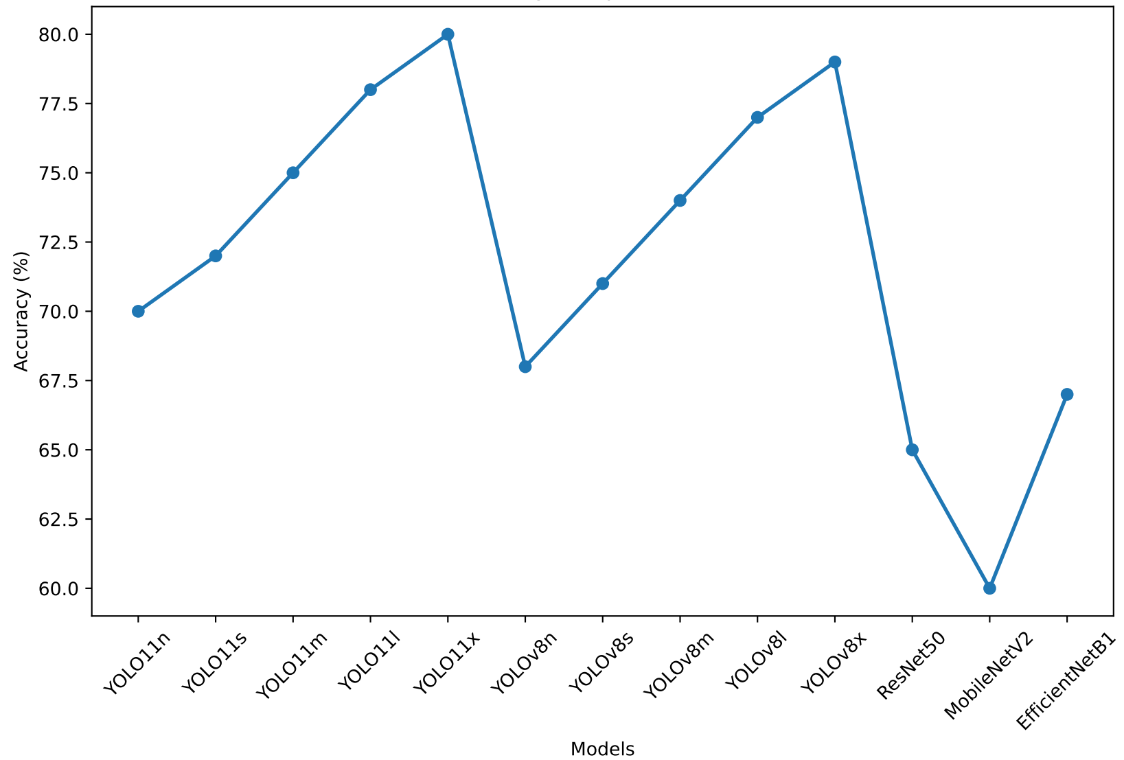
Accuracy Comparison (Line)
