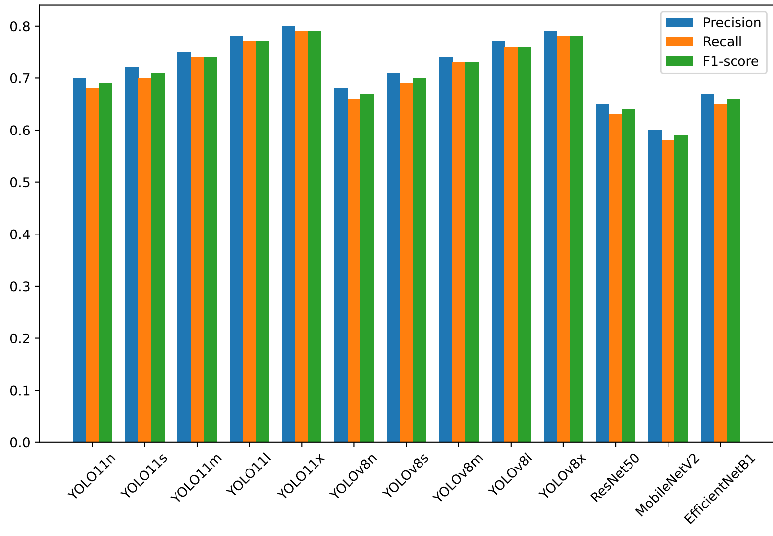
Precision, Recall, F1-score
