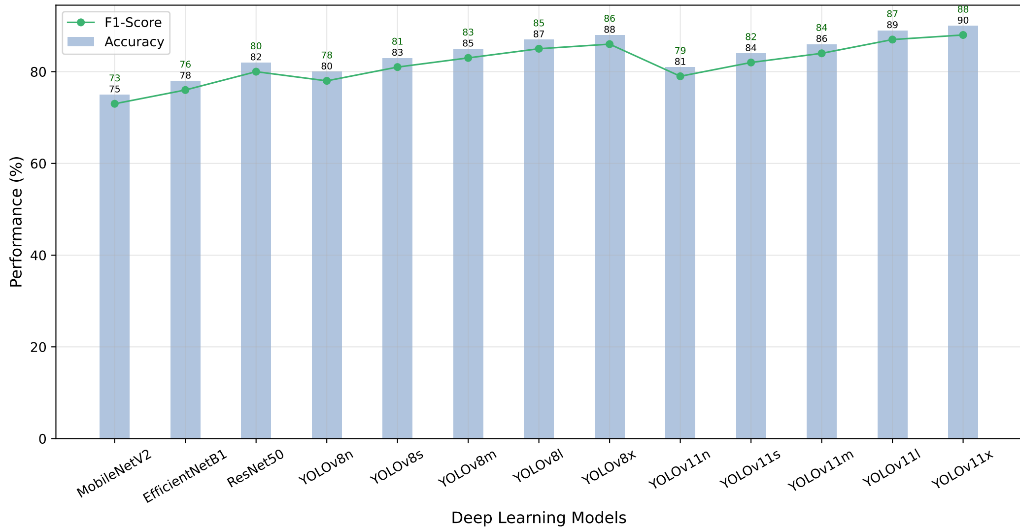
Figure 1: Accuracy and F1-Score Comparison of CNN variants
