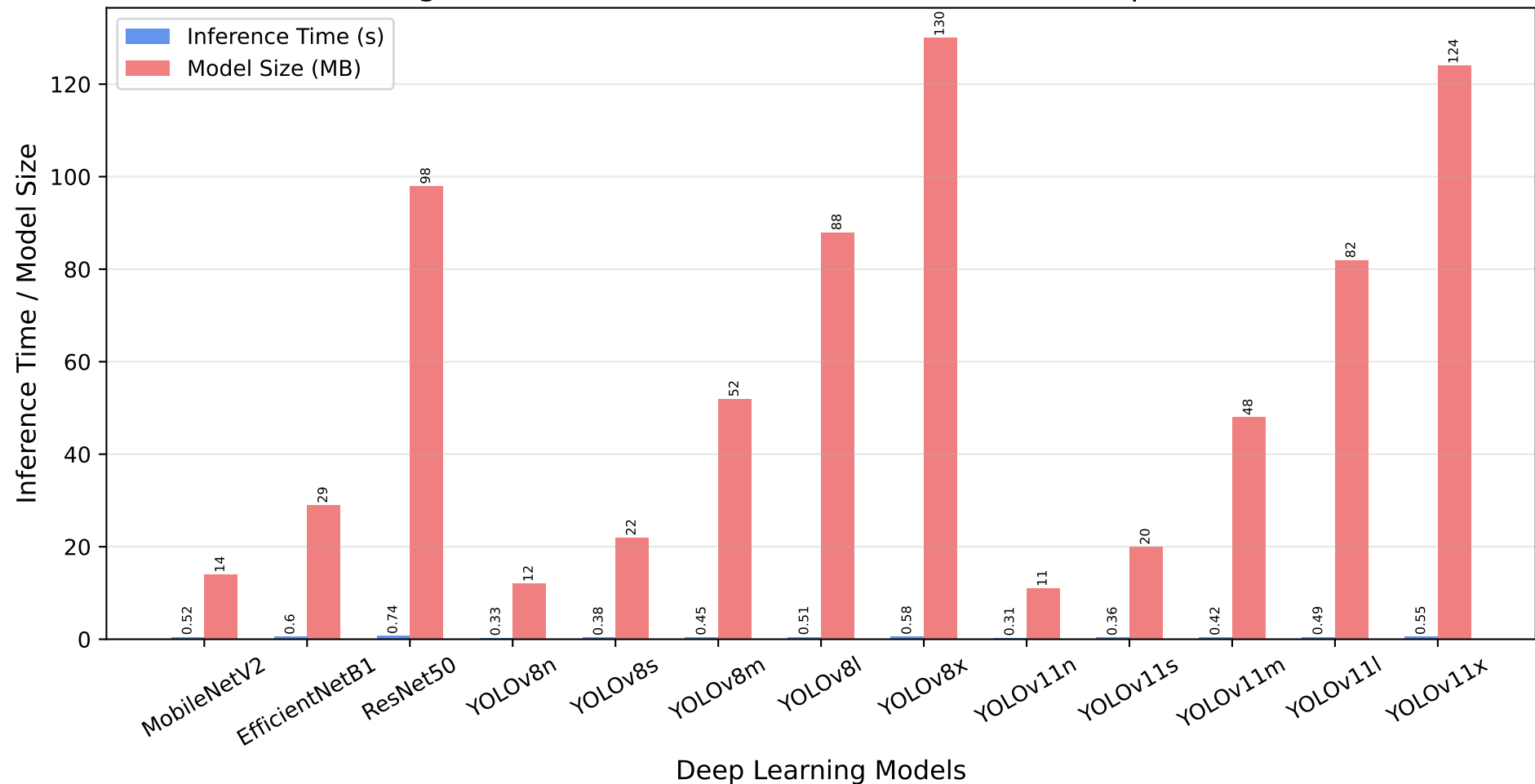
Figure 2: Inference Time and Model Size Comparison
