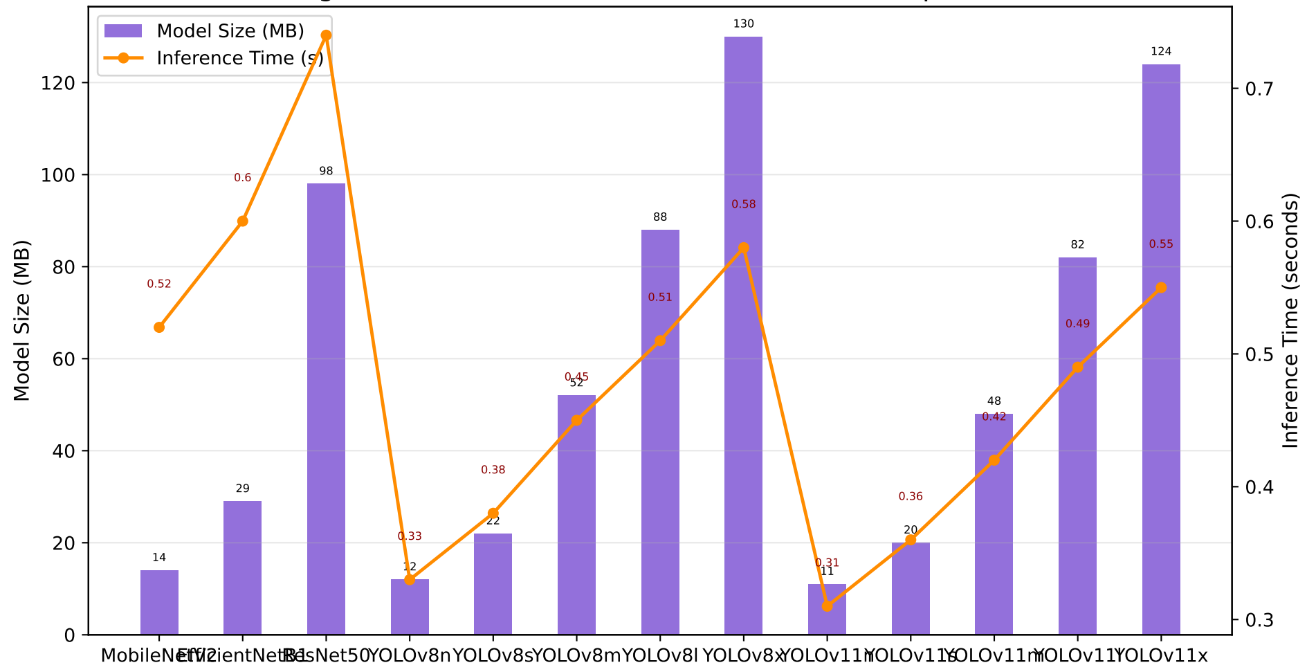
Figure 2: Model Size and Inference Time Comparison
