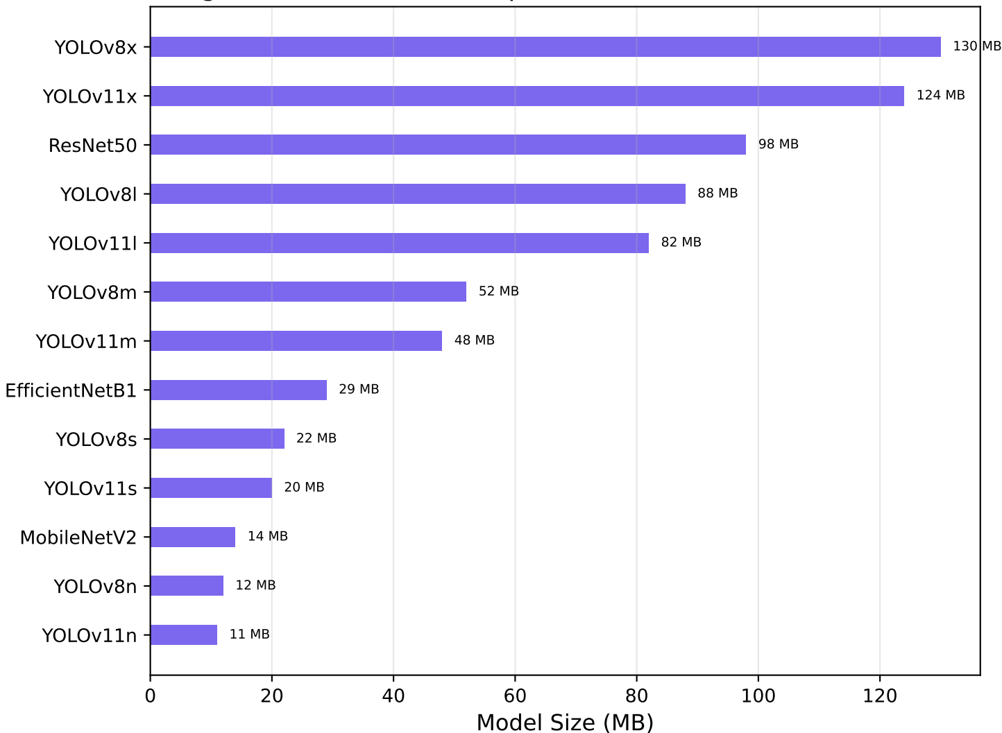
Figure 2: Model Size Comparison of CNN and YOLO Variants
