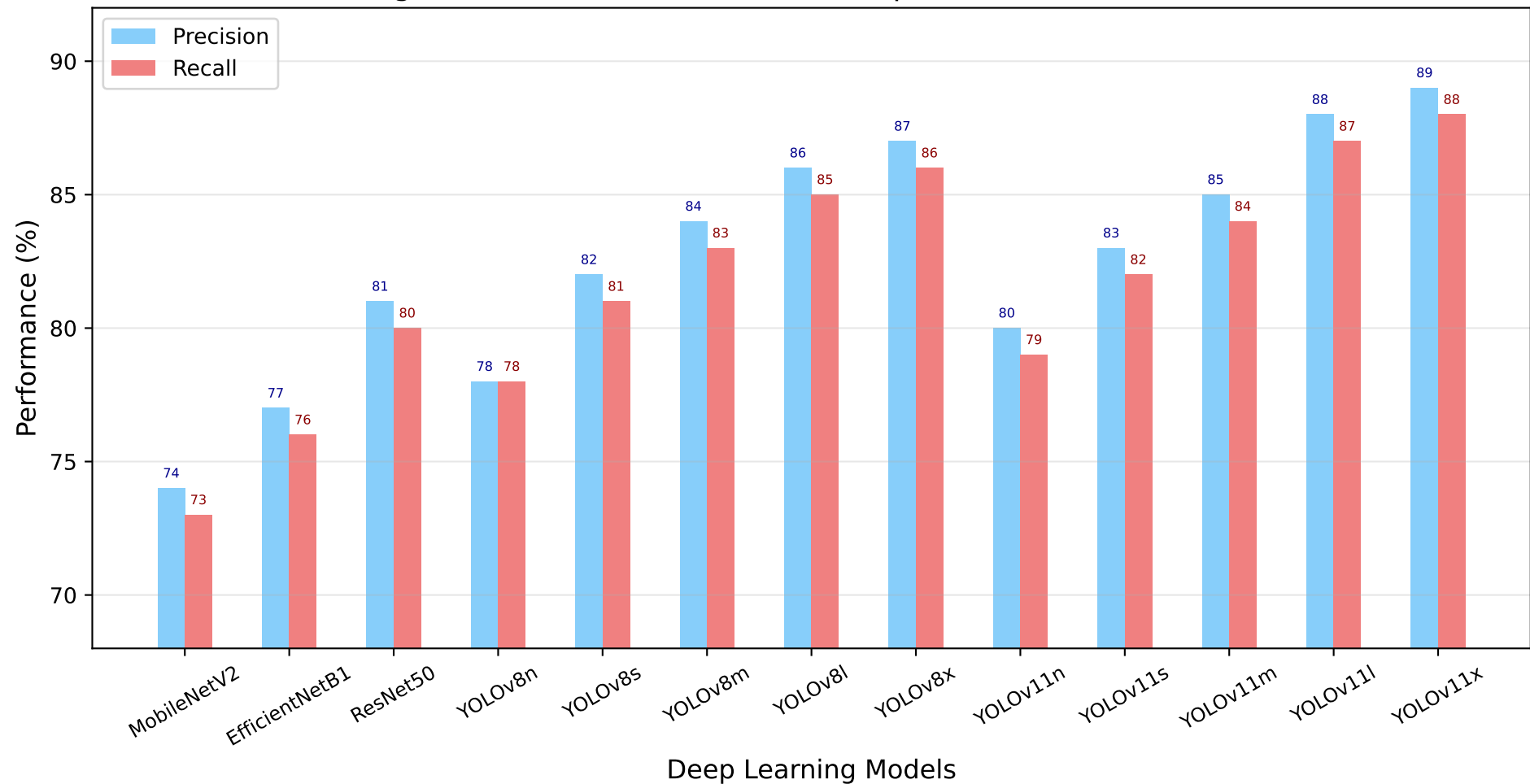
Figure 2: Precision and Recall Comparison of CNN Variants
