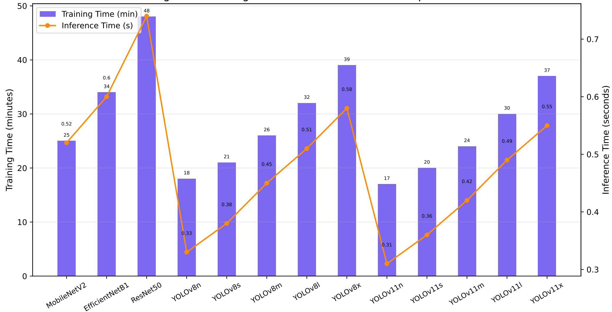
0.74 Figure 3: Training Time and Inference Time Comparison
